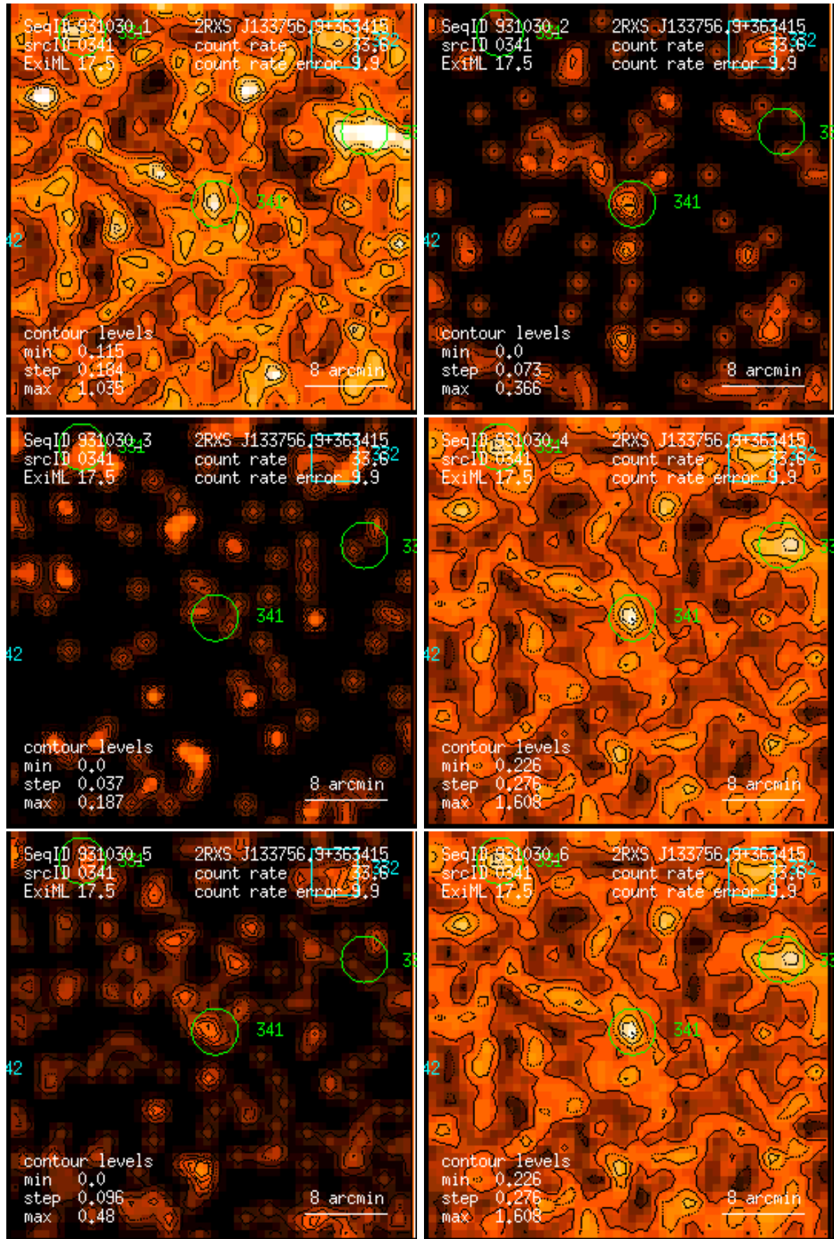
Figure 341: RASS 931030: detection 0341: band rate images, Gaussian filter: (1) PSPC channels 11 – 41, (2) 52 – 90, (3) 91 – 201, (4) 11 – 235, (5) 52 – 201, (6) 11 – 201. Broad band rates in counts/ks. Band rate contour levels in counts/ks/arcmin 2 .
