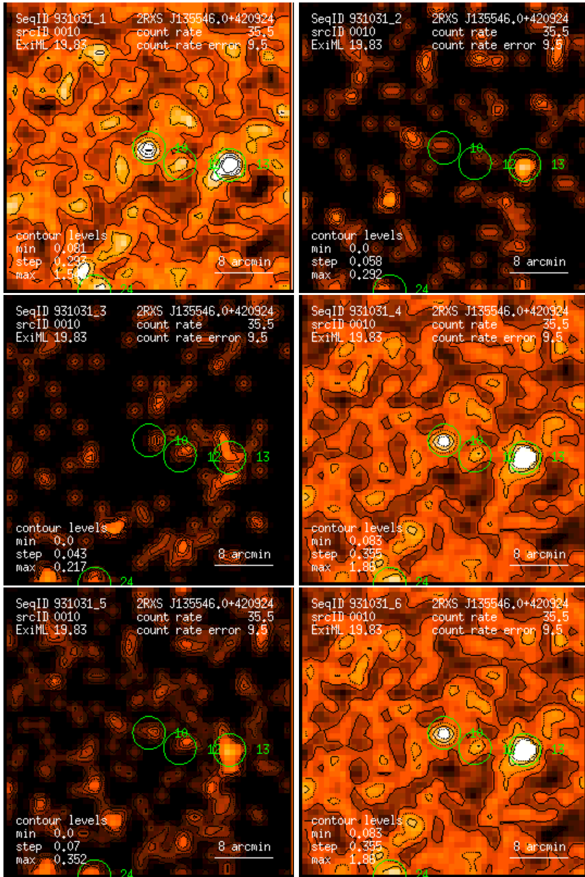
Figure 10: RASS 931031: detection 0010: band rate images, Gaussian filter: (1) PSPC channels 11 – 41, (2) 52 – 90, (3) 91 – 201, (4) 11 – 235, (5) 52 – 201, (6) 11 – 201. Broad band rates in counts/ks. Band rate contour levels in counts/ks/arcmin 2 .
