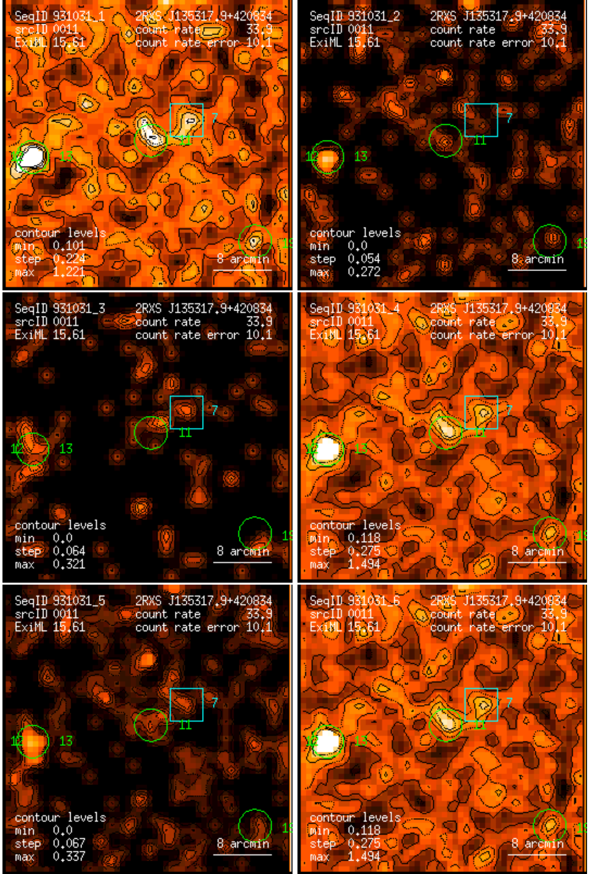
Figure 11: RASS 931031: detection 0011: band rate images, Gaussian filter: (1) PSPC channels 11 – 41, (2) 52 – 90, (3) 91 – 201, (4) 11 – 235, (5) 52 – 201, (6) 11 – 201. Broad band rates in counts/ks. Band rate contour levels in counts/ks/arcmin 2 .
