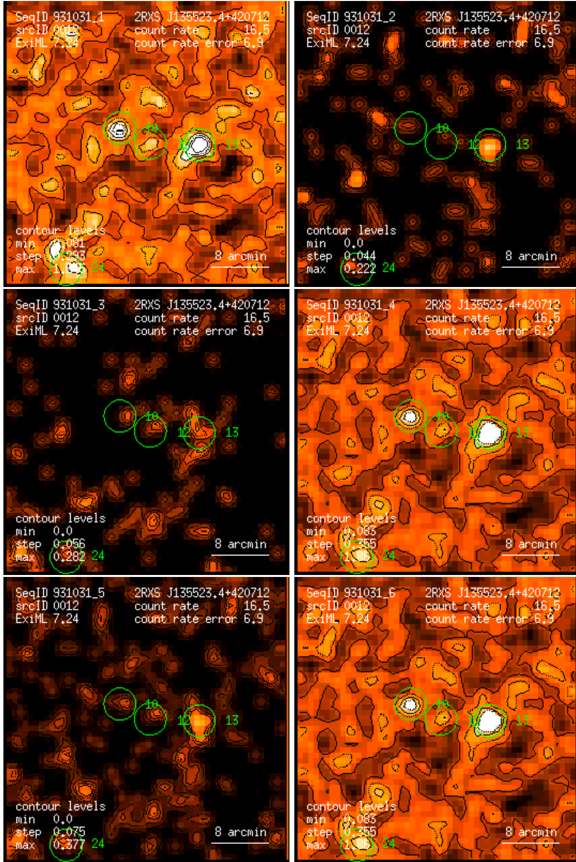
Figure 12: RASS 931031: detection 0012: band rate images, Gaussian filter: (1) PSPC channels 11 – 41, (2) 52 – 90, (3) 91 – 201, (4) 11 – 235, (5) 52 – 201, (6) 11 – 201. Broad band rates in counts/ks. Band rate contour levels in counts/ks/arcmin 2 .
