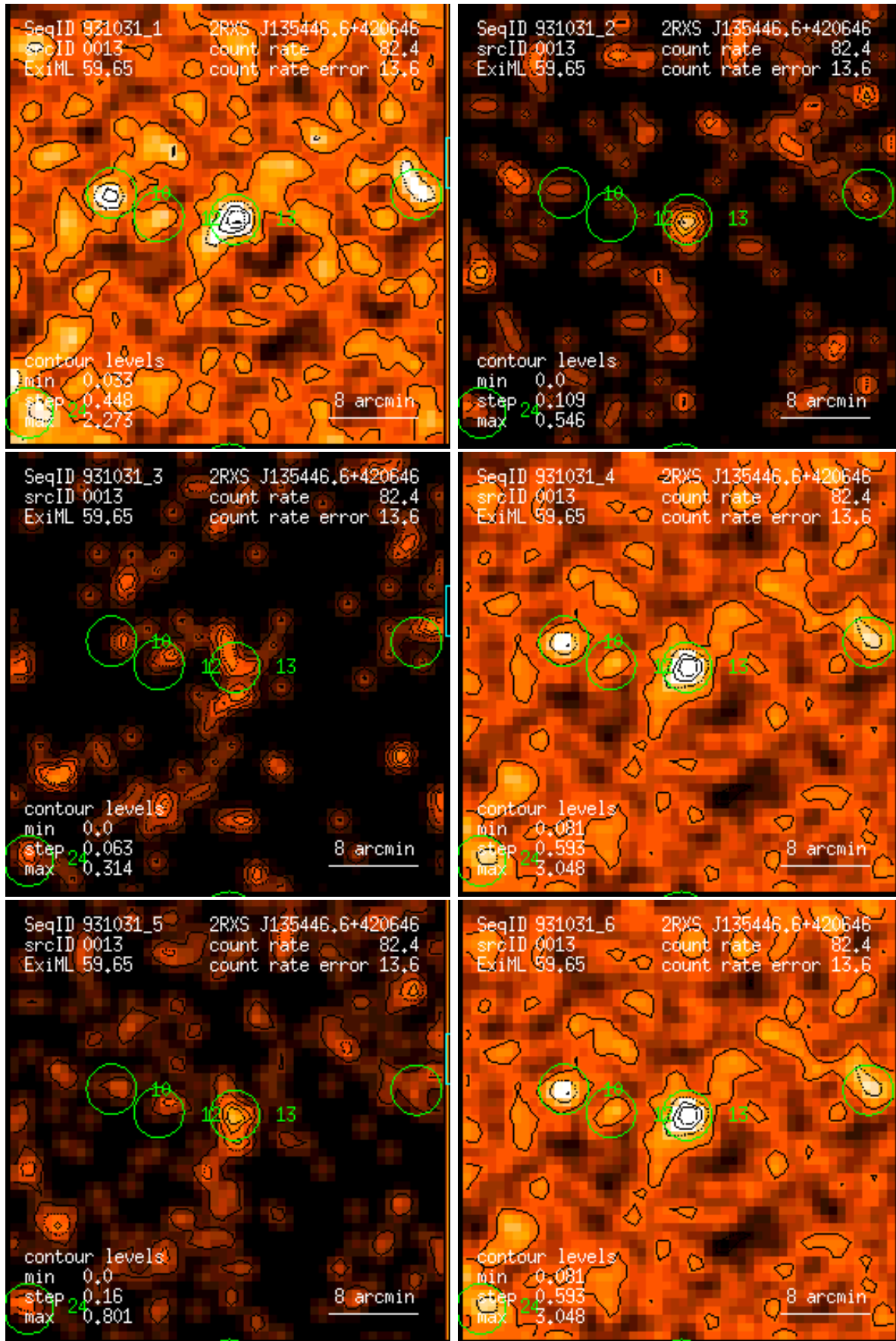
Figure 13: RASS 931031: detection 0013: band rate images, Gaussian filter: (1) PSPC channels 11 – 41, (2) 52 – 90, (3) 91 – 201, (4) 11 – 235, (5) 52 – 201, (6) 11 – 201. Broad band rates in counts/ks. Band rate contour levels in counts/ks/arcmin 2 .
