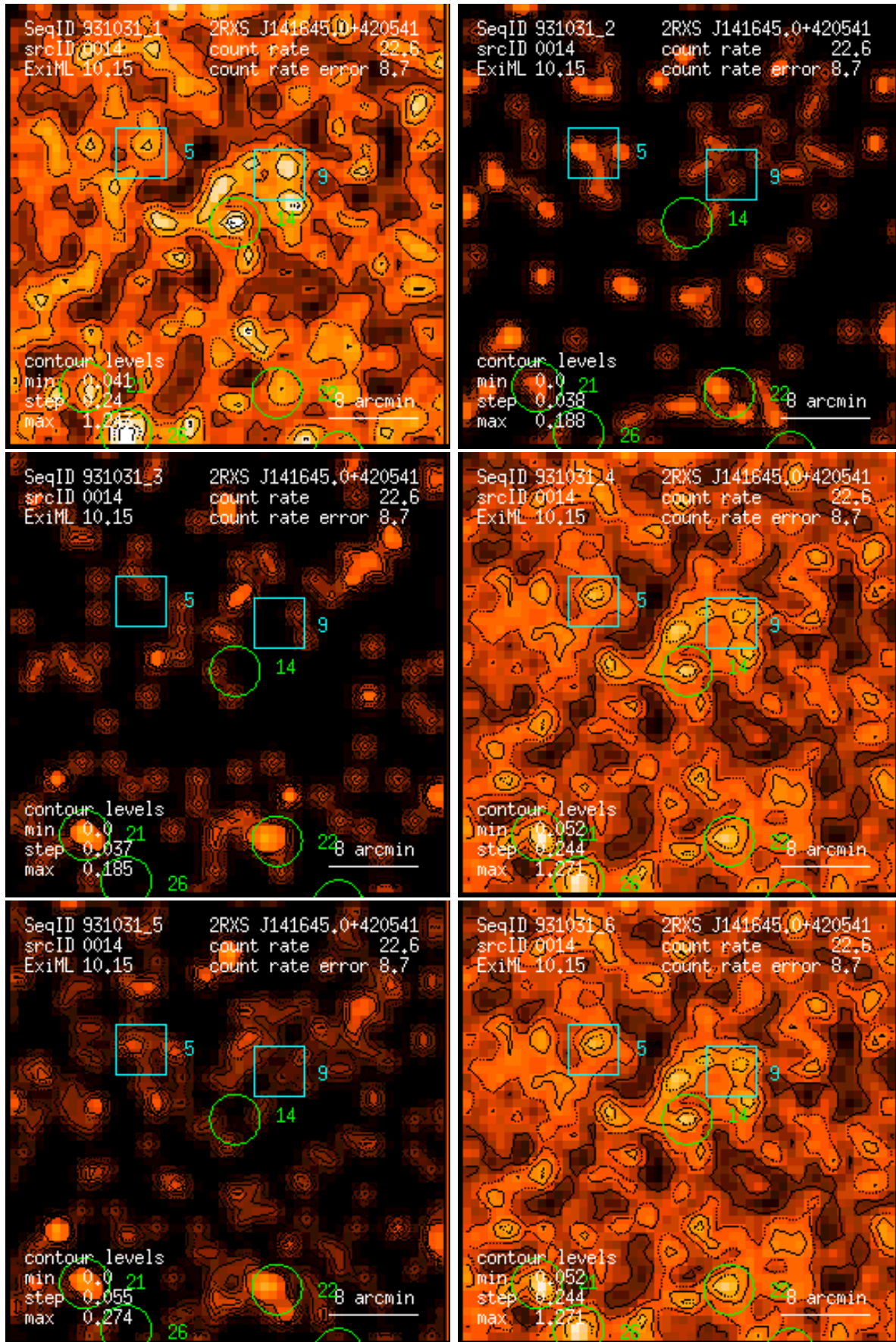
Figure 14: RASS 931031: detection 0014: band rate images, Gaussian filter: (1) PSPC channels 11 – 41, (2) 52 – 90, (3) 91 – 201, (4) 11 – 235, (5) 52 – 201, (6) 11 – 201. Broad band rates in counts/ks. Band rate contour levels in counts/ks/arcmin 2 .
