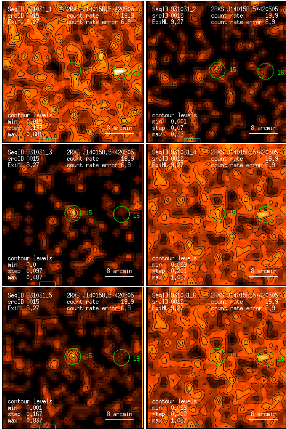
Figure 15: RASS 931031: detection 0015: band rate images, Gaussian filter: (1) PSPC channels 11 – 41, (2) 52 – 90, (3) 91 – 201, (4) 11 – 235, (5) 52 – 201, (6) 11 – 201. Broad band rates in counts/ks. Band rate contour levels in counts/ks/arcmin 2 .
