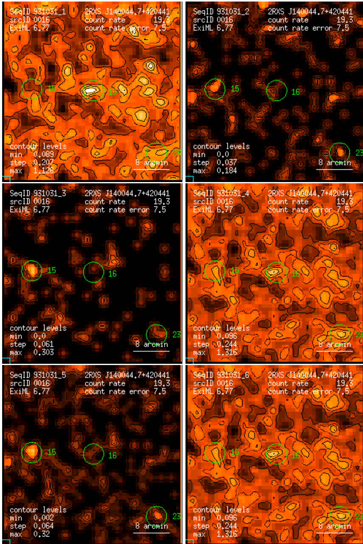
Figure 16: RASS 931031: detection 0016: band rate images, Gaussian filter: (1) PSPC channels 11 – 41, (2) 52 – 90, (3) 91 – 201, (4) 11 – 235, (5) 52 – 201, (6) 11 – 201. Broad band rates in counts/ks. Band rate contour levels in counts/ks/arcmin 2 .
