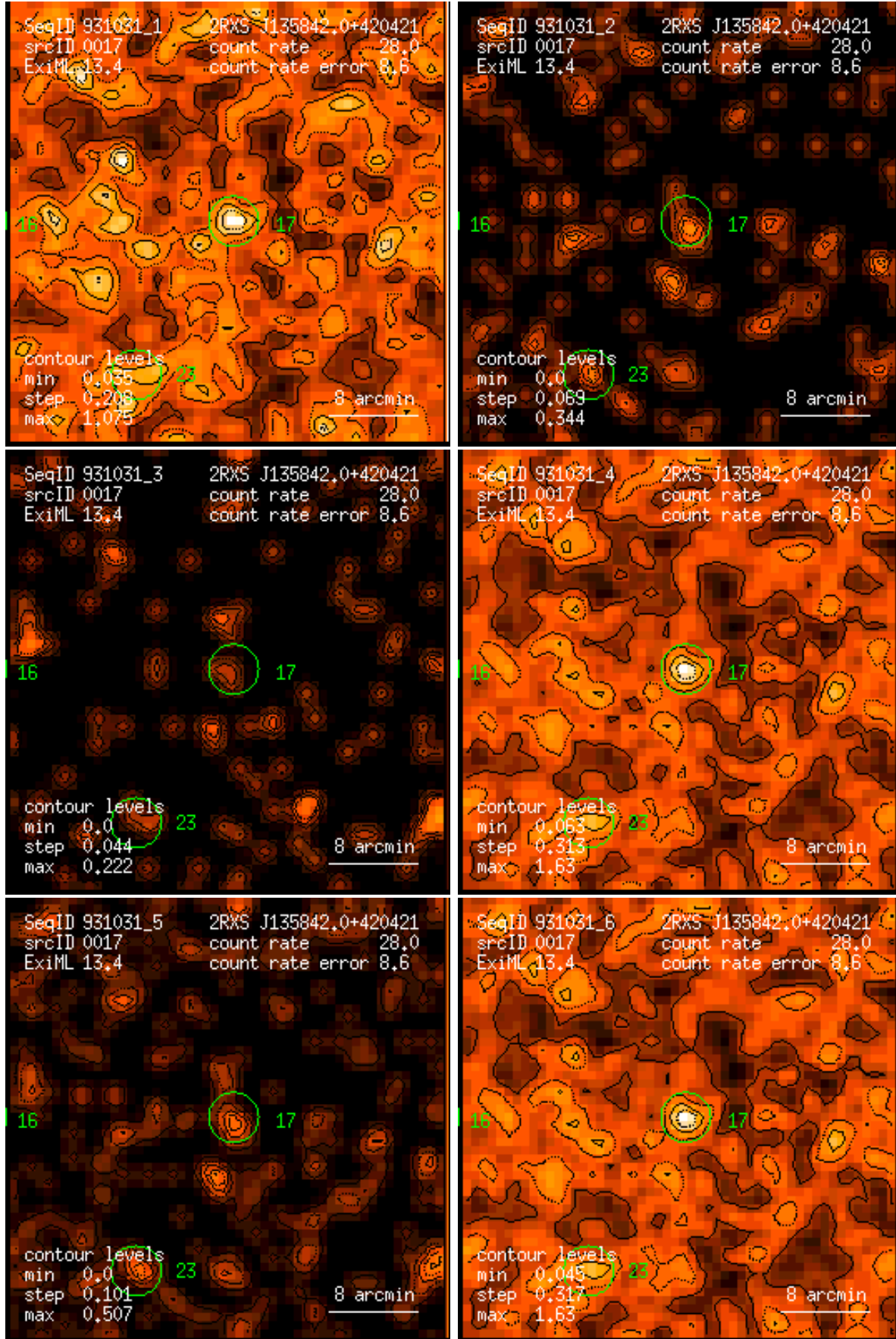
Figure 17: RASS 931031: detection 0017: band rate images, Gaussian filter: (1) PSPC channels 11 – 41, (2) 52 – 90, (3) 91 – 201, (4) 11 – 235, (5) 52 – 201, (6) 11 – 201. Broad band rates in counts/ks. Band rate contour levels in counts/ks/arcmin 2 .
