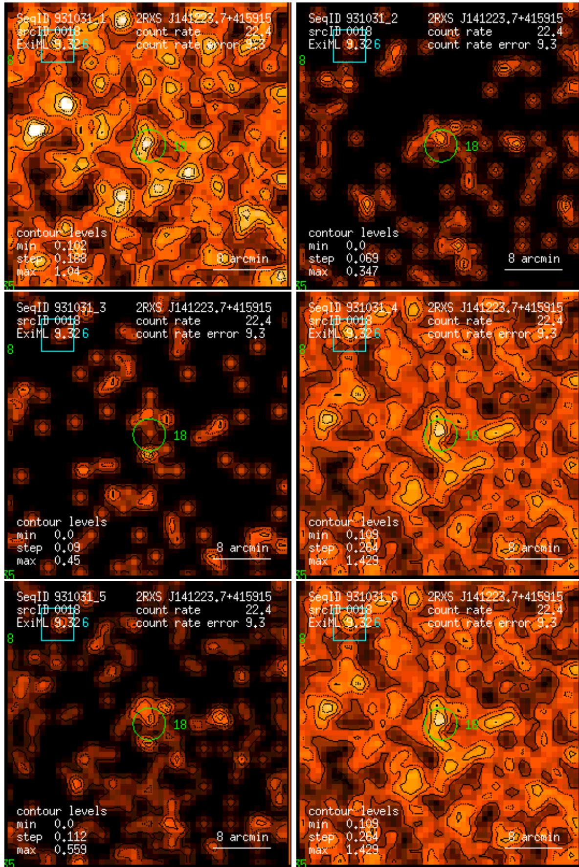
Figure 18: RASS 931031: detection 0018: band rate images, Gaussian filter: (1) PSPC channels 11 – 41, (2) 52 – 90, (3) 91 – 201, (4) 11 – 235, (5) 52 – 201, (6) 11 – 201. Broad band rates in counts/ks. Band rate contour levels in counts/ks/arcmin 2 .
