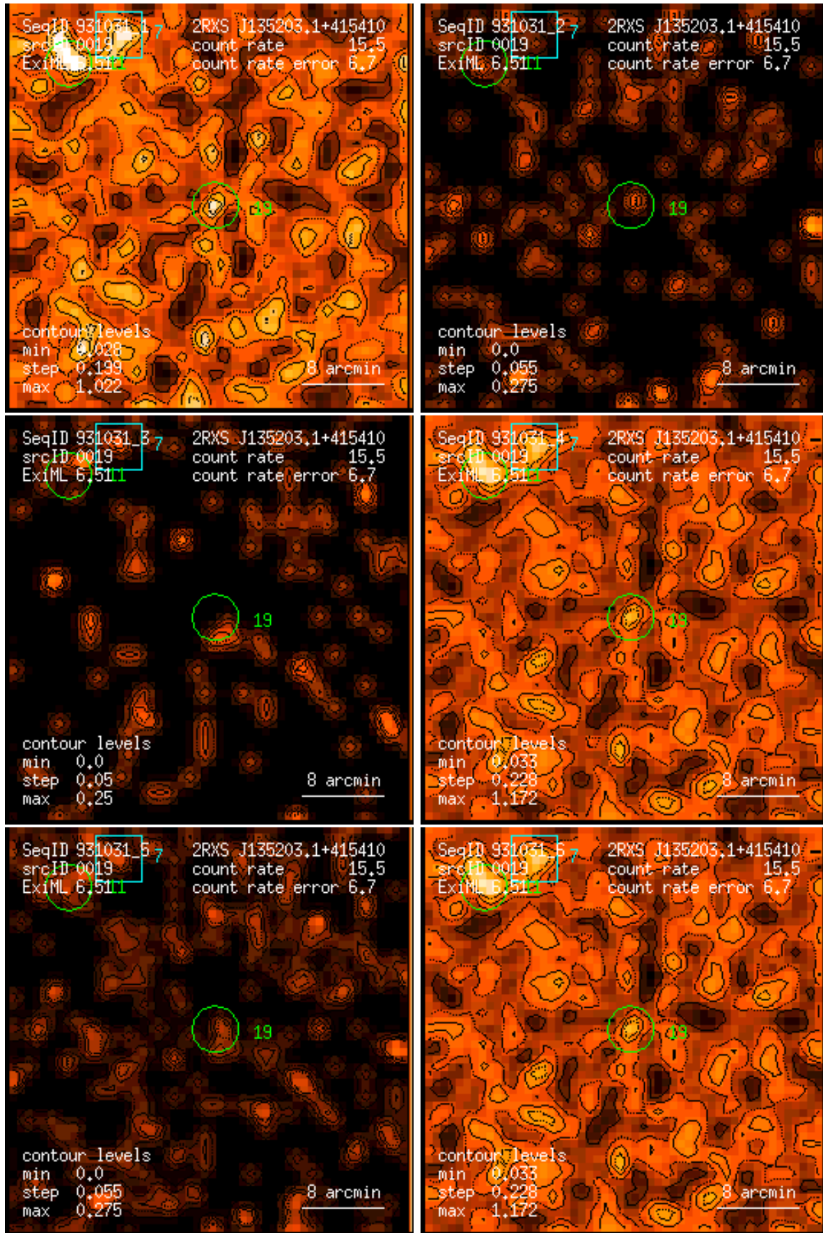
Figure 19: RASS 931031: detection 0019: band rate images, Gaussian filter: (1) PSPC channels 11 – 41, (2) 52 – 90, (3) 91 – 201, (4) 11 – 235, (5) 52 – 201, (6) 11 – 201. Broad band rates in counts/ks. Band rate contour levels in counts/ks/arcmin 2 .
