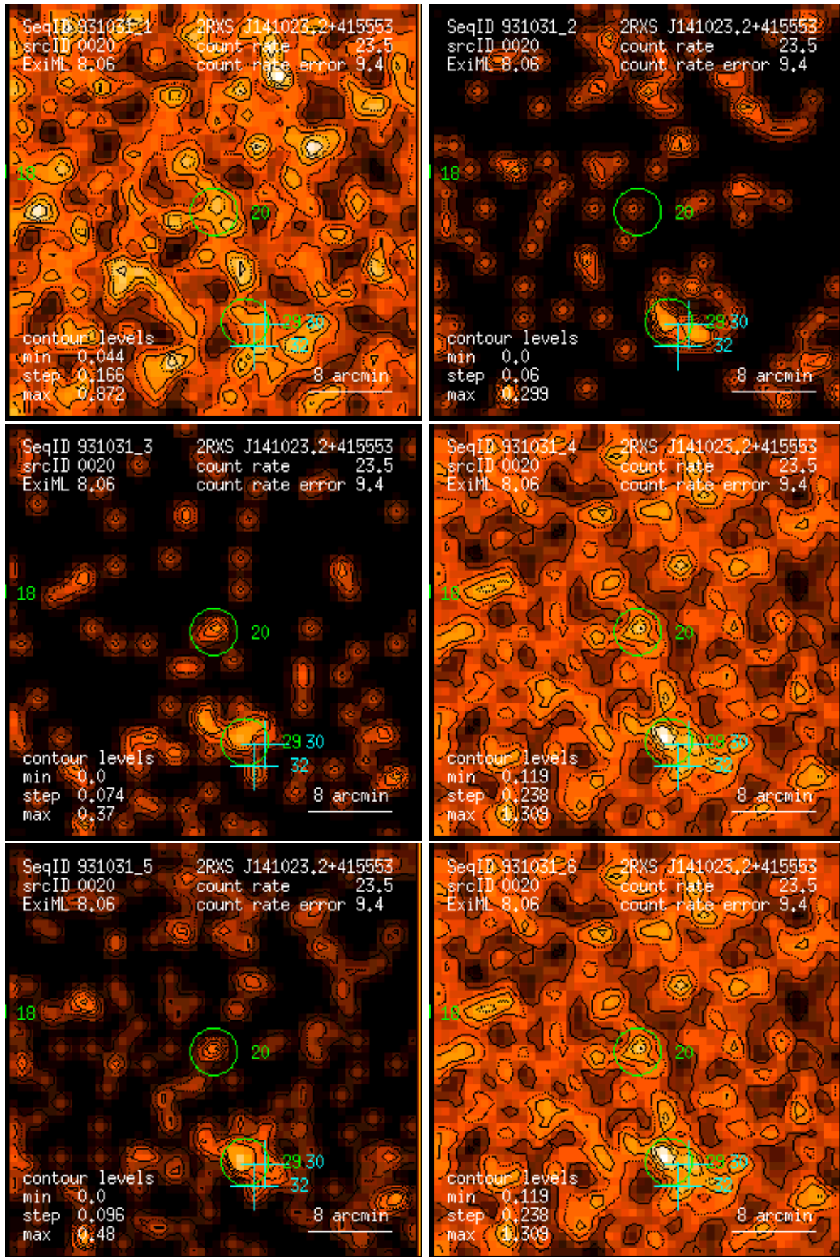
Figure 20: RASS 931031: detection 0020: band rate images, Gaussian filter: (1) PSPC channels 11 – 41, (2) 52 – 90, (3) 91 – 201, (4) 11 – 235, (5) 52 – 201, (6) 11 – 201. Broad band rates in counts/ks. Band rate contour levels in counts/ks/arcmin 2 .
