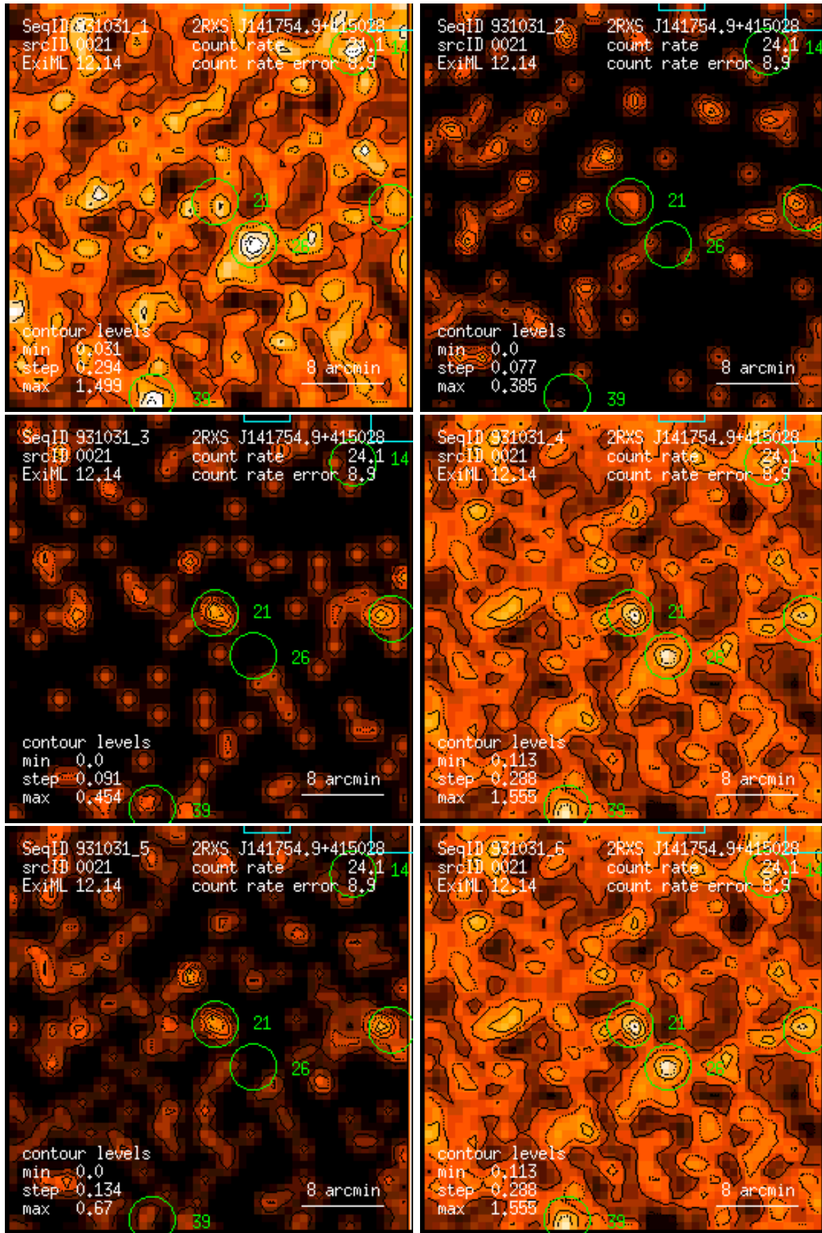
Figure 21: RASS 931031: detection 0021: band rate images, Gaussian filter: (1) PSPC channels 11 – 41, (2) 52 – 90, (3) 91 – 201, (4) 11 – 235, (5) 52 – 201, (6) 11 – 201. Broad band rates in counts/ks. Band rate contour levels in counts/ks/arcmin 2 .
