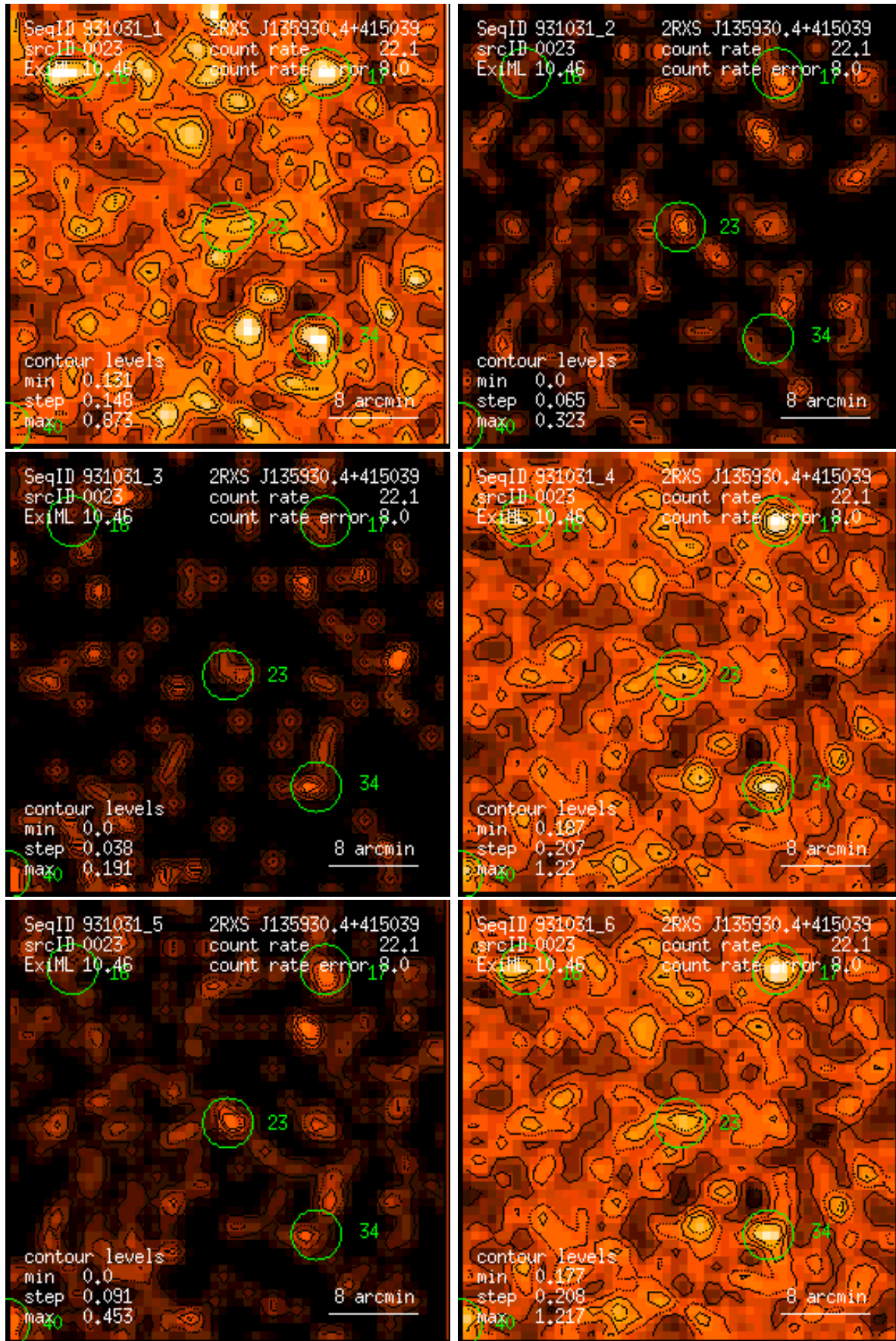
Figure 23: RASS 931031: detection 0023: band rate images, Gaussian filter: (1) PSPC channels 11 – 41, (2) 52 – 90, (3) 91 – 201, (4) 11 – 235, (5) 52 – 201, (6) 11 – 201. Broad band rates in counts/ks. Band rate contour levels in counts/ks/arcmin 2 .
