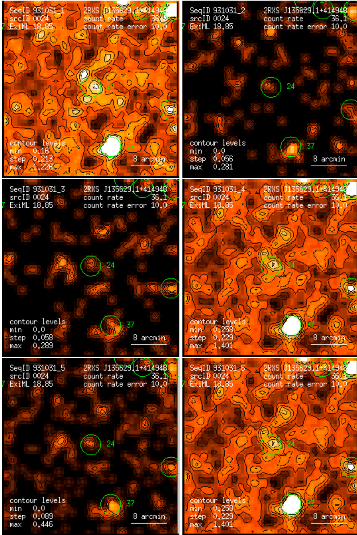
Figure 24: RASS 931031: detection 0024: band rate images, Gaussian filter: (1) PSPC channels 11 – 41, (2) 52 – 90, (3) 91 – 201, (4) 11 – 235, (5) 52 – 201, (6) 11 – 201. Broad band rates in counts/ks. Band rate contour levels in counts/ks/arcmin 2 .
