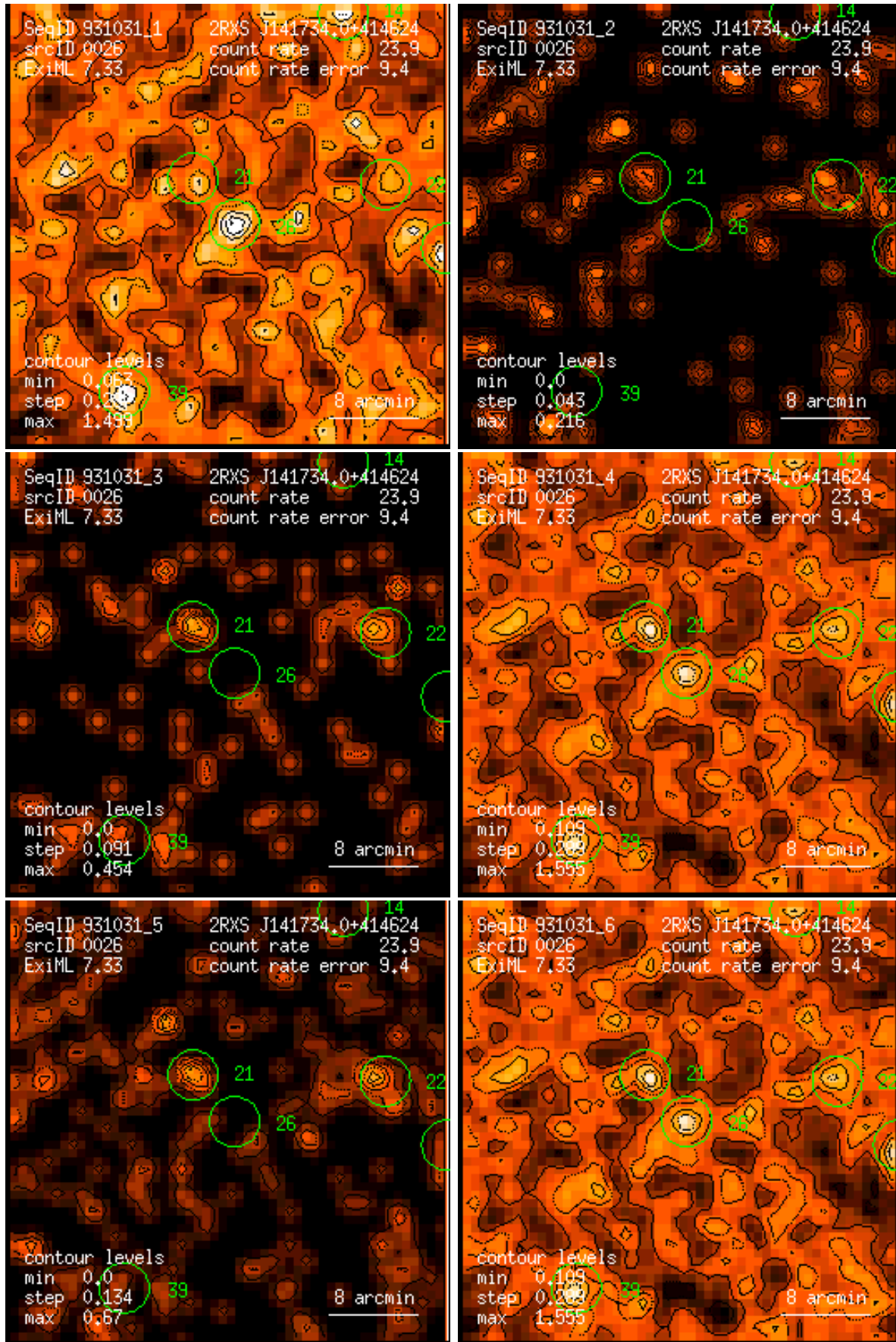
Figure 26: RASS 931031: detection 0026: band rate images, Gaussian filter: (1) PSPC channels 11 – 41, (2) 52 – 90, (3) 91 – 201, (4) 11 – 235, (5) 52 – 201, (6) 11 – 201. Broad band rates in counts/ks. Band rate contour levels in counts/ks/arcmin 2 .
