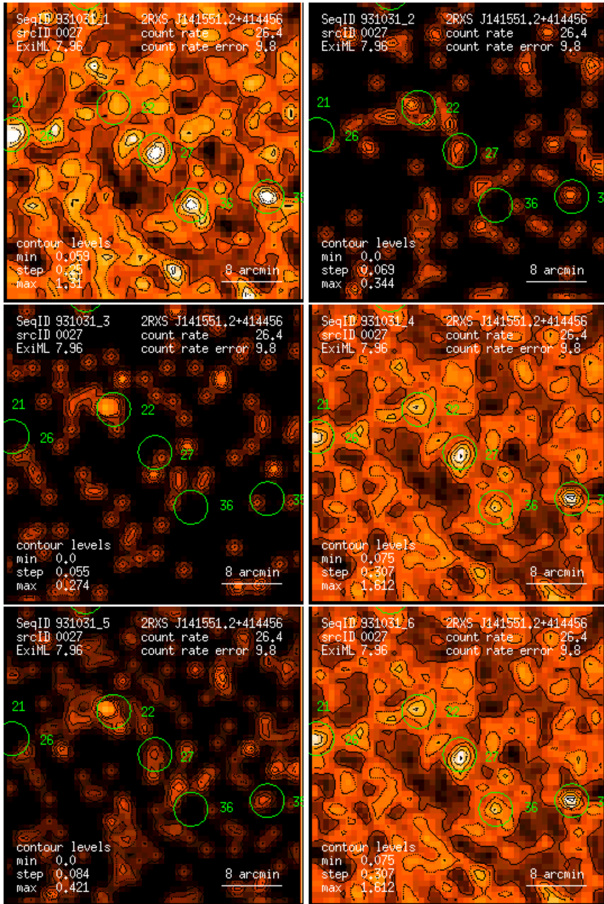
Figure 27: RASS 931031: detection 0027: band rate images, Gaussian filter: (1) PSPC channels 11 – 41, (2) 52 – 90, (3) 91 – 201, (4) 11 – 235, (5) 52 – 201, (6) 11 – 201. Broad band rates in counts/ks. Band rate contour levels in counts/ks/arcmin 2 .
