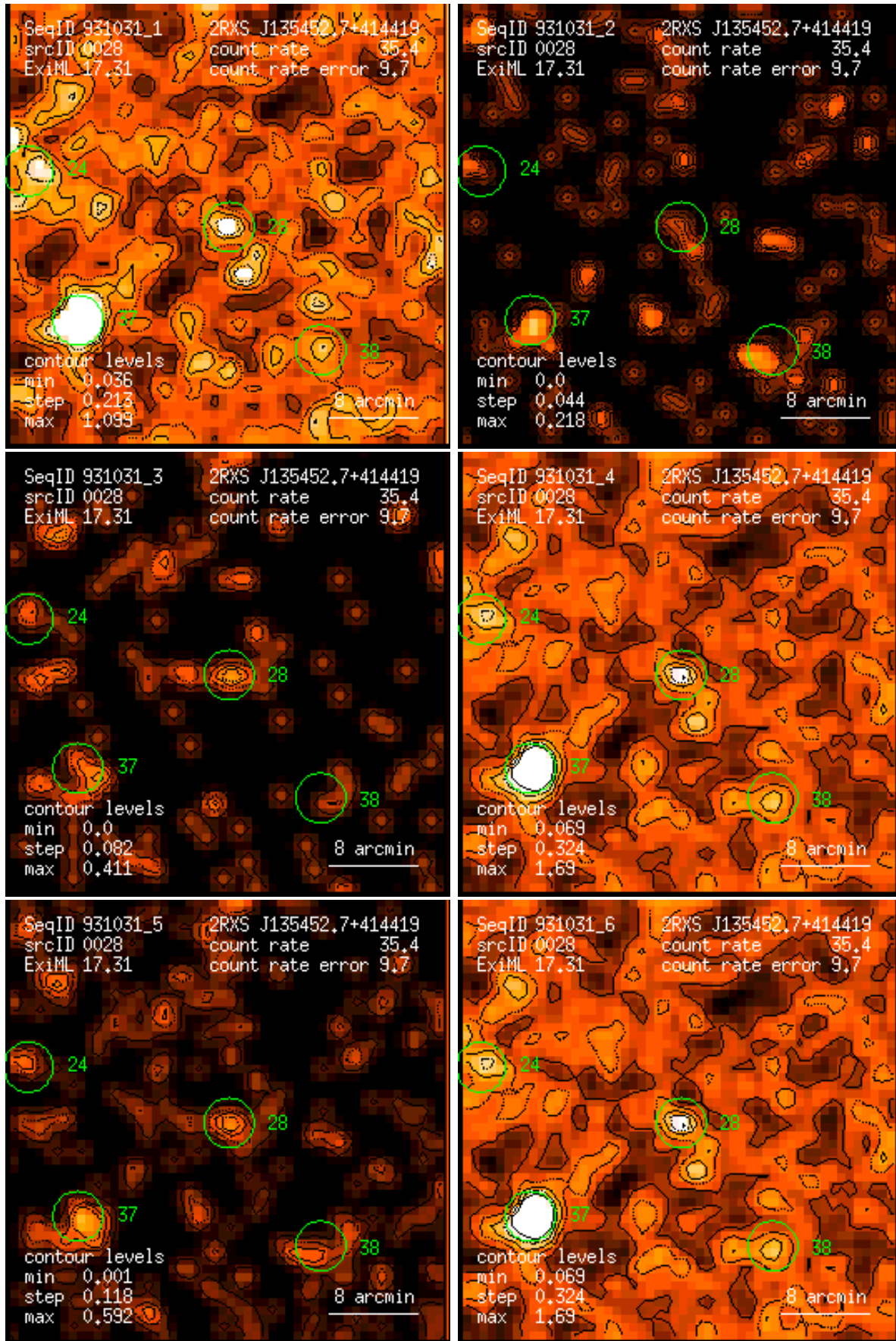
Figure 28: RASS 931031: detection 0028: band rate images, Gaussian filter: (1) PSPC channels 11 – 41, (2) 52 – 90, (3) 91 – 201, (4) 11 – 235, (5) 52 – 201, (6) 11 – 201. Broad band rates in counts/ks. Band rate contour levels in counts/ks/arcmin 2 .
