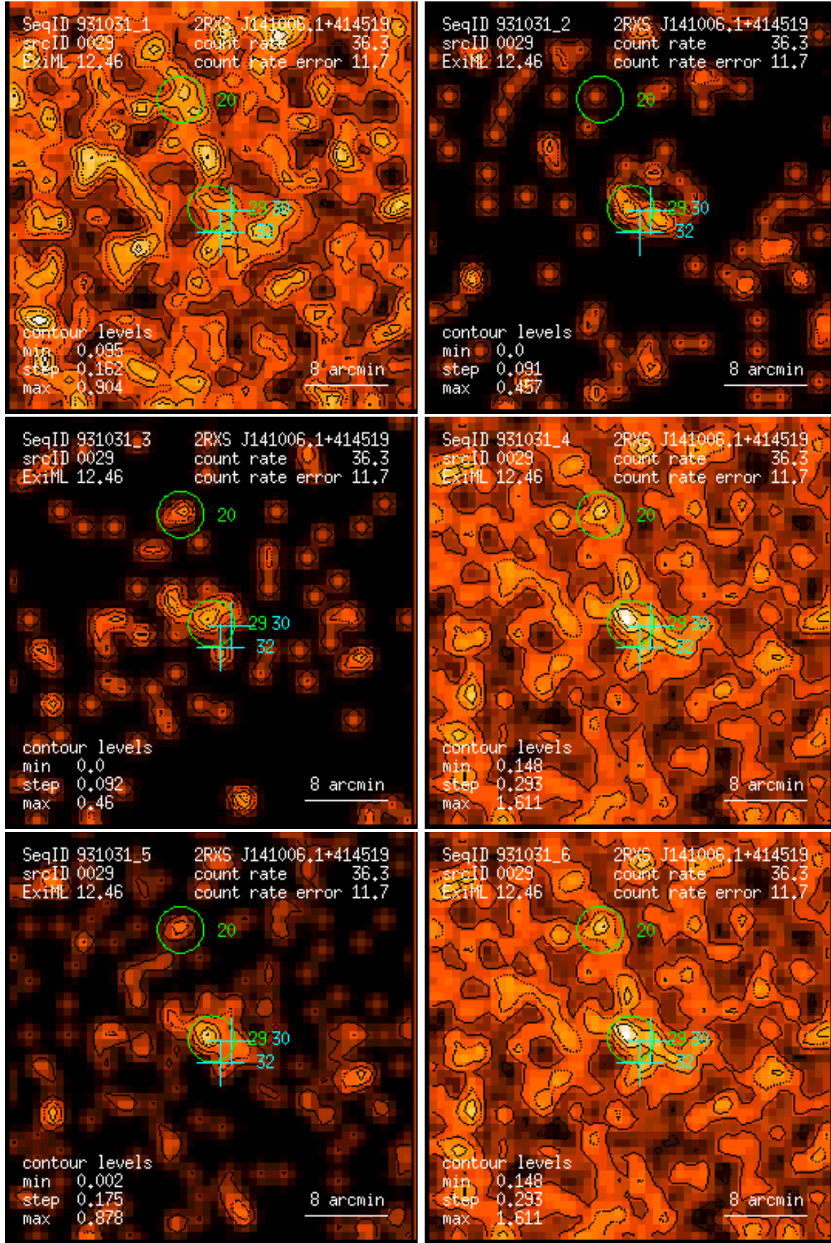
Figure 29: RASS 931031: detection 0029: band rate images, Gaussian filter: (1) PSPC channels 11 – 41, (2) 52 – 90, (3) 91 – 201, (4) 11 – 235, (5) 52 – 201, (6) 11 – 201. Broad band rates in counts/ks. Band rate contour levels in counts/ks/arcmin 2 .
