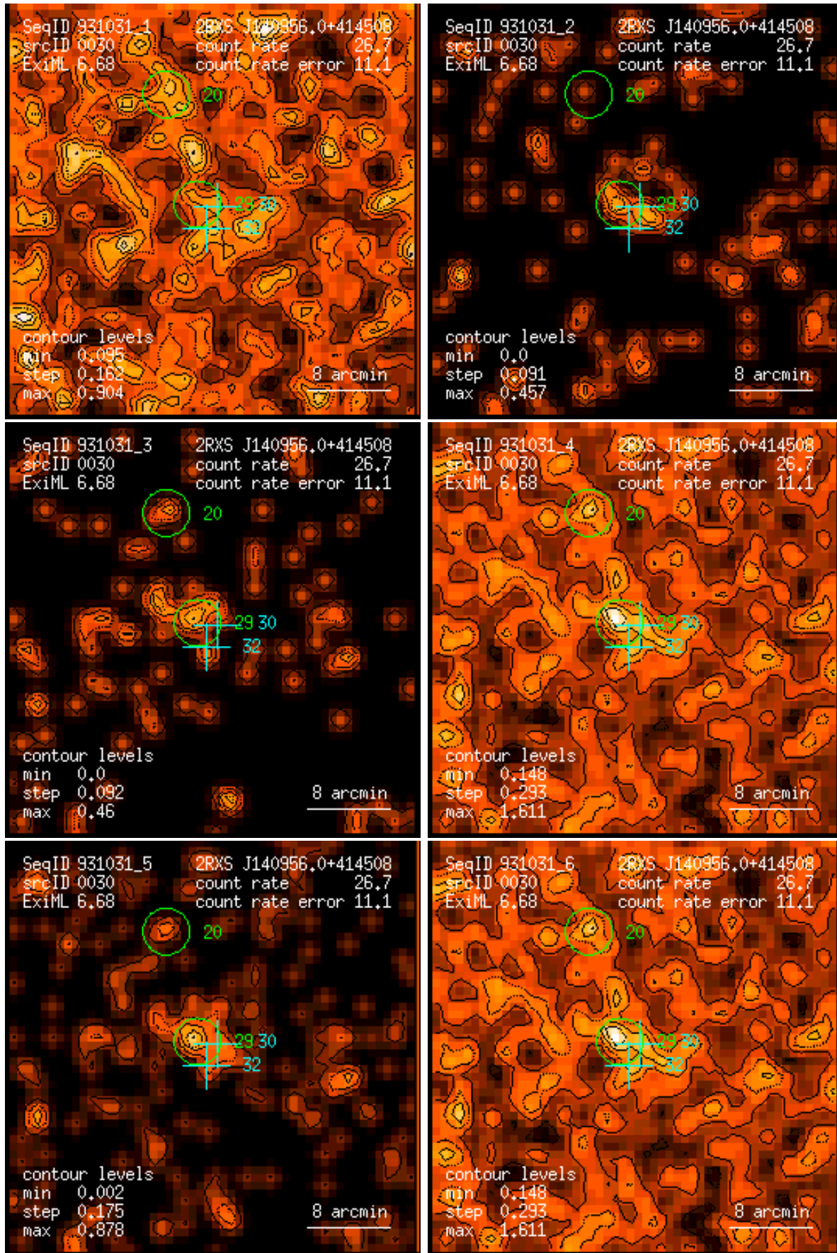
Figure 30: RASS 931031: detection 0030: band rate images, Gaussian filter: (1) PSPC channels 11 – 41, (2) 52 – 90, (3) 91 – 201, (4) 11 – 235, (5) 52 – 201, (6) 11 – 201. Broad band rates in counts/ks. Band rate contour levels in counts/ks/arcmin 2 .
