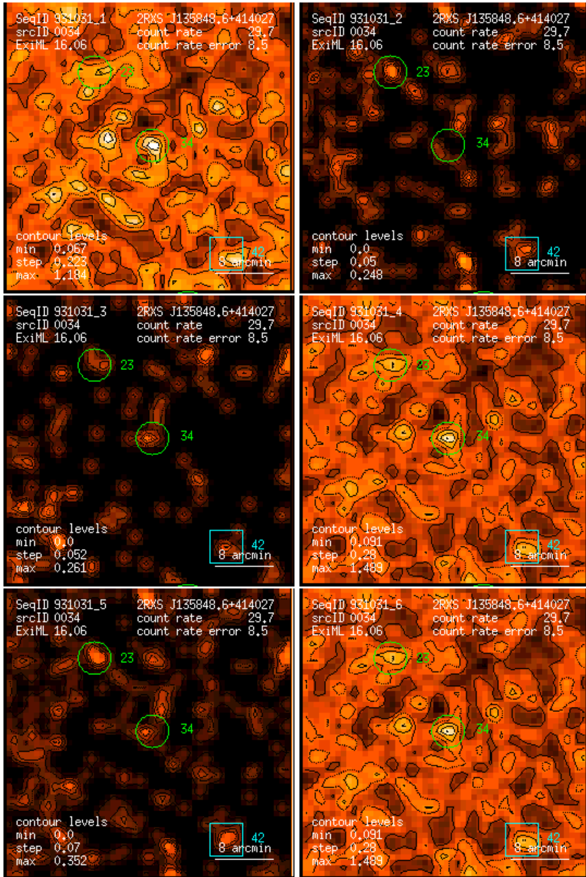
Figure 34: RASS 931031: detection 0034: band rate images, Gaussian filter: (1) PSPC channels 11 – 41, (2) 52 – 90, (3) 91 – 201, (4) 11 – 235, (5) 52 – 201, (6) 11 – 201. Broad band rates in counts/ks. Band rate contour levels in counts/ks/arcmin 2 .
