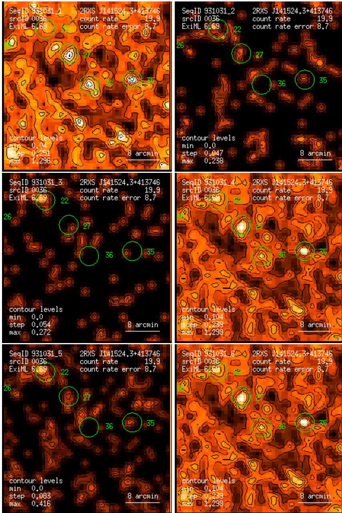
Figure 36: RASS 931031: detection 0036: band rate images, Gaussian filter: (1) PSPC channels 11 – 41, (2) 52 – 90, (3) 91 – 201, (4) 11 – 235, (5) 52 – 201, (6) 11 – 201. Broad band rates in counts/ks. Band rate contour levels in counts/ks/arcmin 2 .
