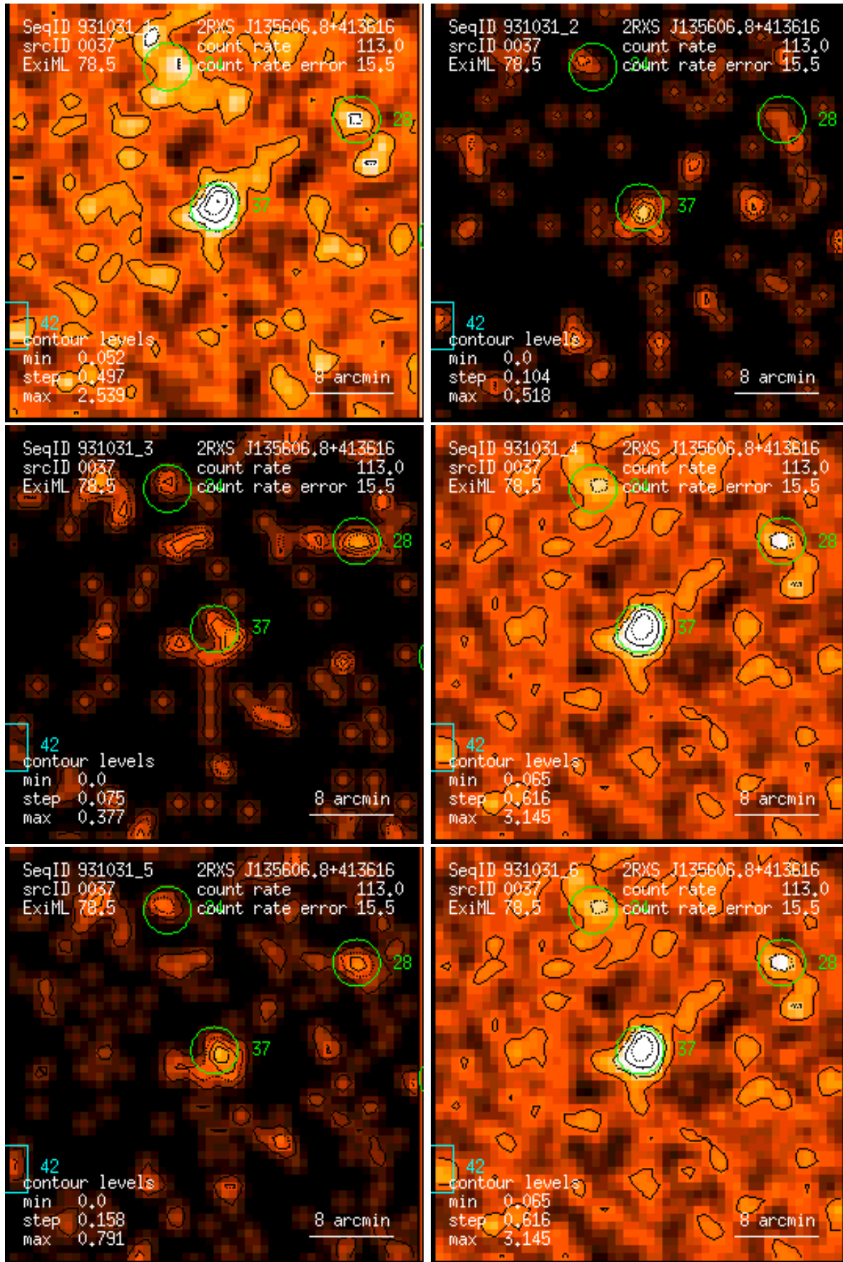
Figure 37: RASS 931031: detection 0037: band rate images, Gaussian filter: (1) PSPC channels 11 – 41, (2) 52 – 90, (3) 91 – 201, (4) 11 – 235, (5) 52 – 201, (6) 11 – 201. Broad band rates in counts/ks. Band rate contour levels in counts/ks/arcmin 2 .
