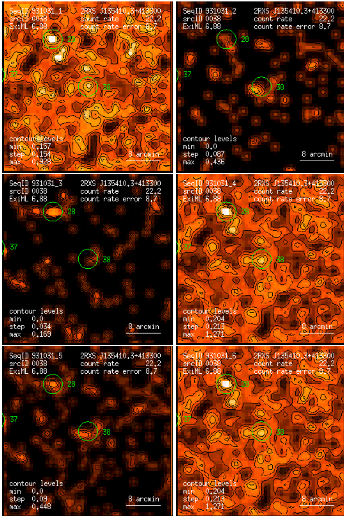
Figure 38: RASS 931031: detection 0038: band rate images, Gaussian filter: (1) PSPC channels 11 – 41, (2) 52 – 90, (3) 91 – 201, (4) 11 – 235, (5) 52 – 201, (6) 11 – 201. Broad band rates in counts/ks. Band rate contour levels in counts/ks/arcmin 2 .
