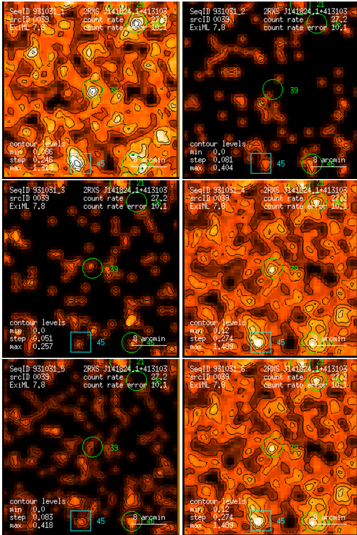
Figure 39: RASS 931031: detection 0039: band rate images, Gaussian filter: (1) PSPC channels 11 – 41, (2) 52 – 90, (3) 91 – 201, (4) 11 – 235, (5) 52 – 201, (6) 11 – 201. Broad band rates in counts/ks. Band rate contour levels in counts/ks/arcmin 2 .
