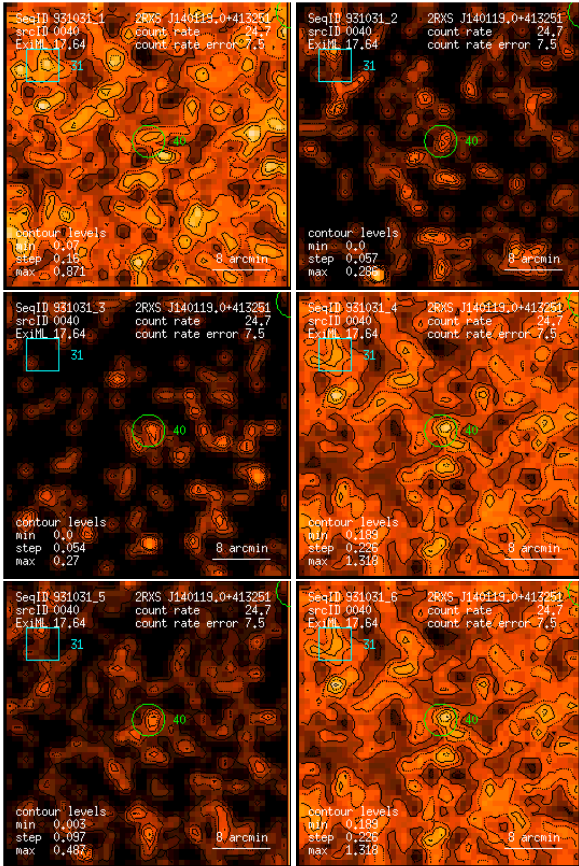
Figure 40: RASS 931031: detection 0040: band rate images, Gaussian filter: (1) PSPC channels 11 – 41, (2) 52 – 90, (3) 91 – 201, (4) 11 – 235, (5) 52 – 201, (6) 11 – 201. Broad band rates in counts/ks. Band rate contour levels in counts/ks/arcmin 2 .
