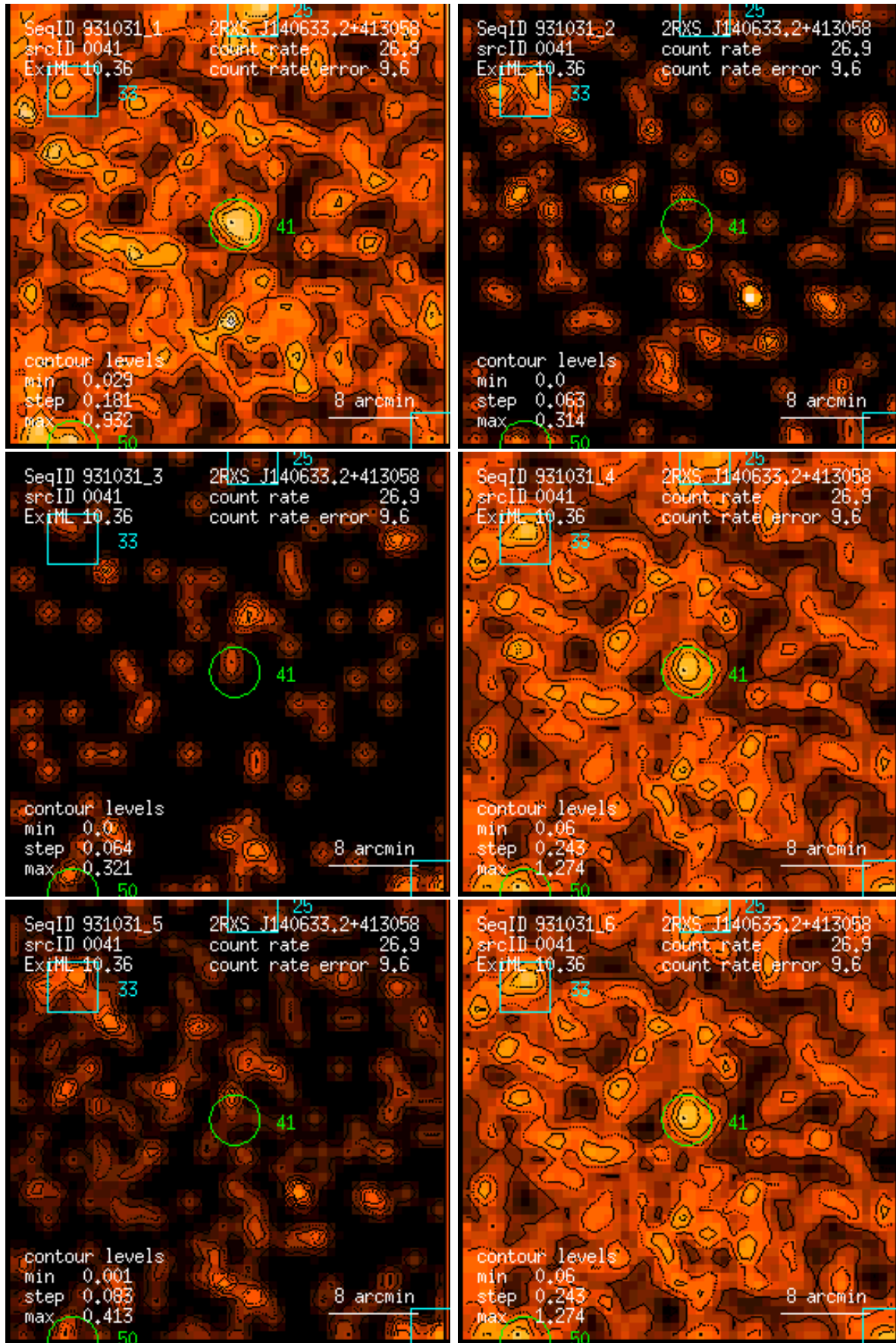
Figure 41: RASS 931031: detection 0041: band rate images, Gaussian filter: (1) PSPC channels 11 – 41, (2) 52 – 90, (3) 91 – 201, (4) 11 – 235, (5) 52 – 201, (6) 11 – 201. Broad band rates in counts/ks. Band rate contour levels in counts/ks/arcmin 2 .
