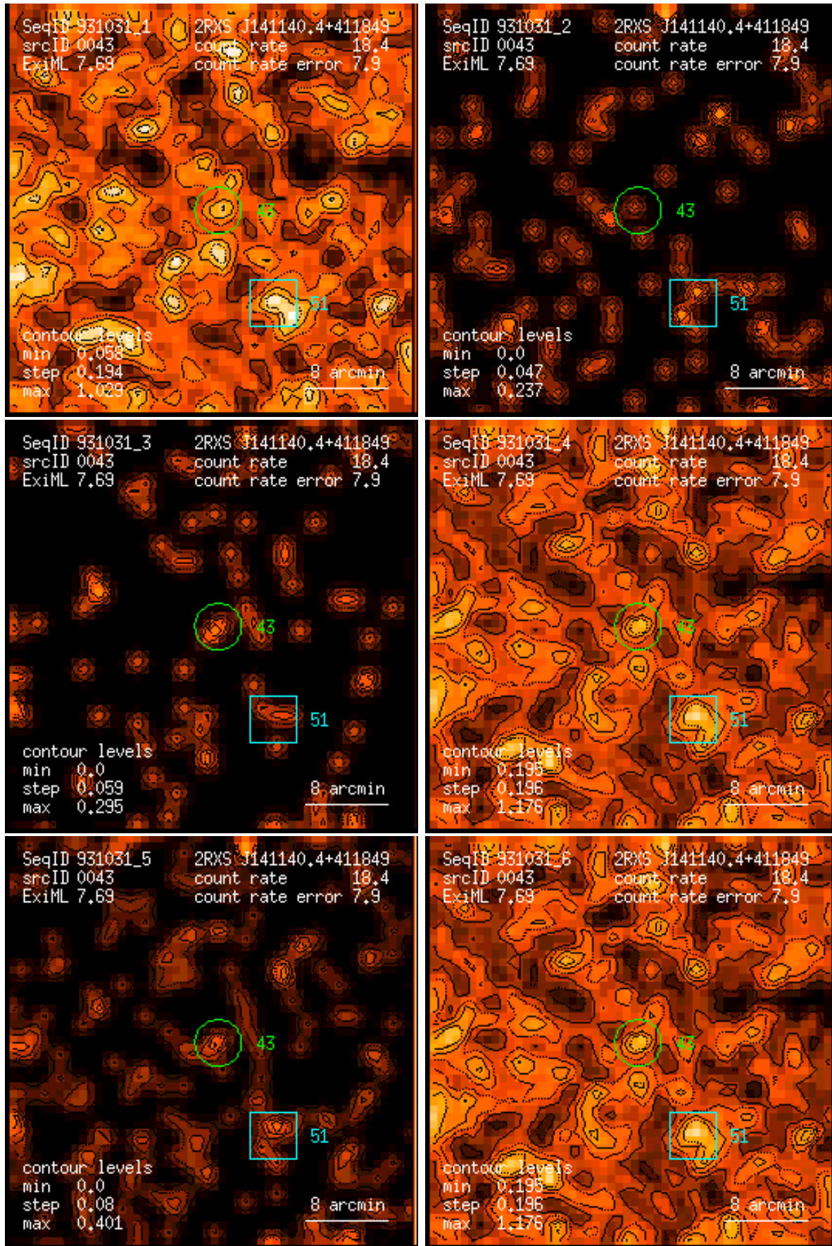
Figure 43: RASS 931031: detection 0043: band rate images, Gaussian filter: (1) PSPC channels 11 – 41, (2) 52 – 90, (3) 91 – 201, (4) 11 – 235, (5) 52 – 201, (6) 11 – 201. Broad band rates in counts/ks. Band rate contour levels in counts/ks/arcmin 2 .
