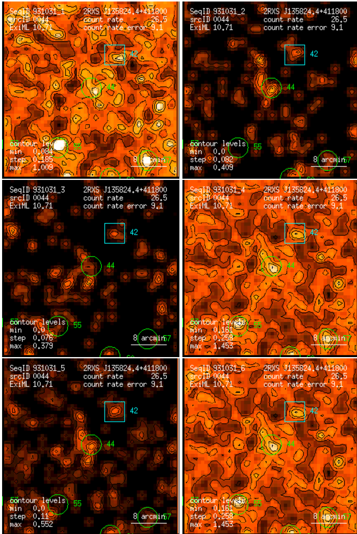
Figure 44: RASS 931031: detection 0044: band rate images, Gaussian filter: (1) PSPC channels 11 – 41, (2) 52 – 90, (3) 91 – 201, (4) 11 – 235, (5) 52 – 201, (6) 11 – 201. Broad band rates in counts/ks. Band rate contour levels in counts/ks/arcmin 2 .
