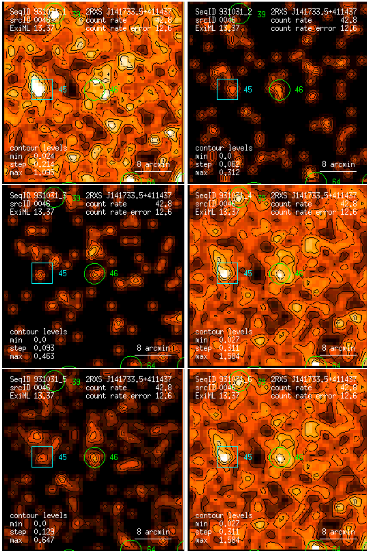
Figure 46: RASS 931031: detection 0046: band rate images, Gaussian filter: (1) PSPC channels 11 – 41, (2) 52 – 90, (3) 91 – 201, (4) 11 – 235, (5) 52 – 201, (6) 11 – 201. Broad band rates in counts/ks. Band rate contour levels in counts/ks/arcmin 2 .
