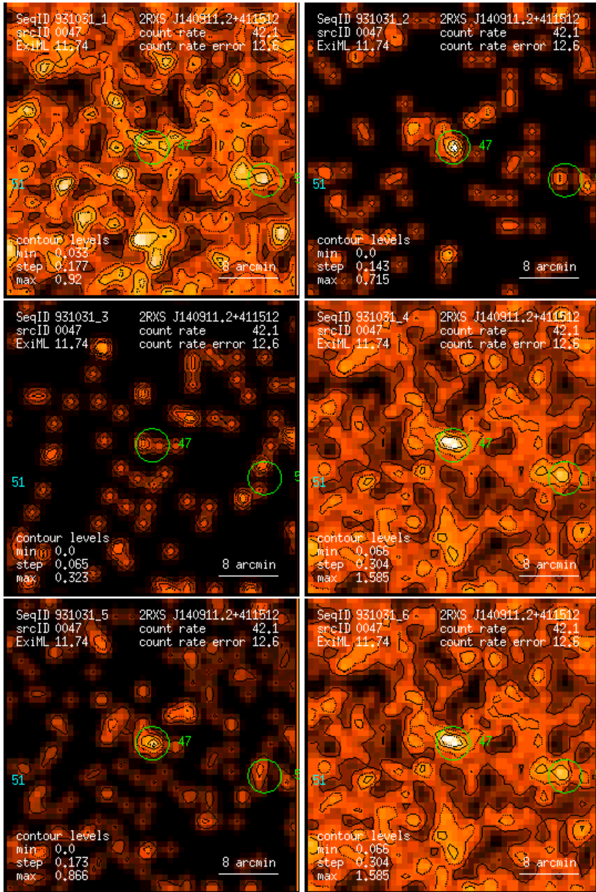
Figure 47: RASS 931031: detection 0047: band rate images, Gaussian filter: (1) PSPC channels 11 – 41, (2) 52 – 90, (3) 91 – 201, (4) 11 – 235, (5) 52 – 201, (6) 11 – 201. Broad band rates in counts/ks. Band rate contour levels in counts/ks/arcmin 2 .
