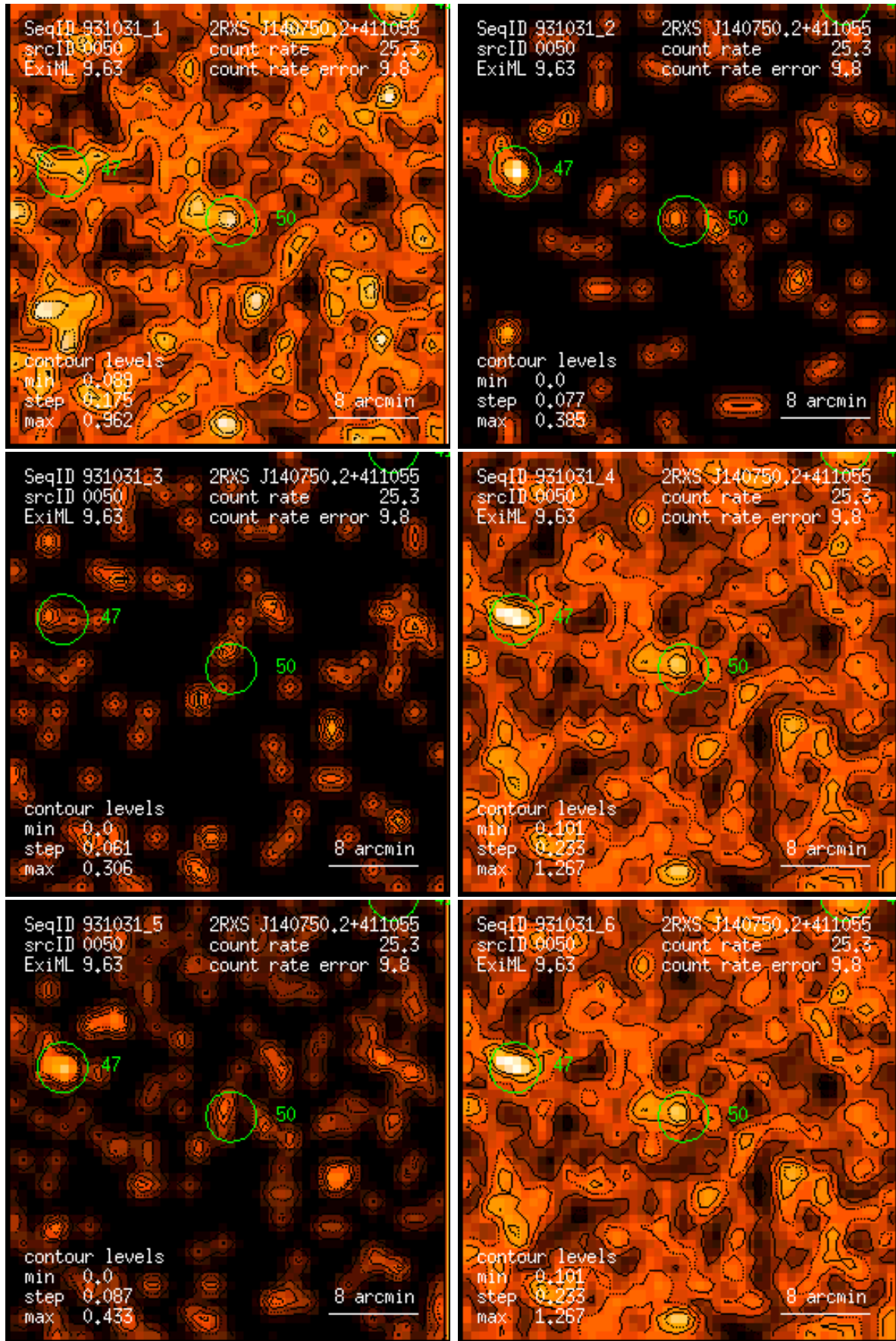
Figure 50: RASS 931031: detection 0050: band rate images, Gaussian filter: (1) PSPC channels 11 – 41, (2) 52 – 90, (3) 91 – 201, (4) 11 – 235, (5) 52 – 201, (6) 11 – 201. Broad band rates in counts/ks. Band rate contour levels in counts/ks/arcmin 2 .
