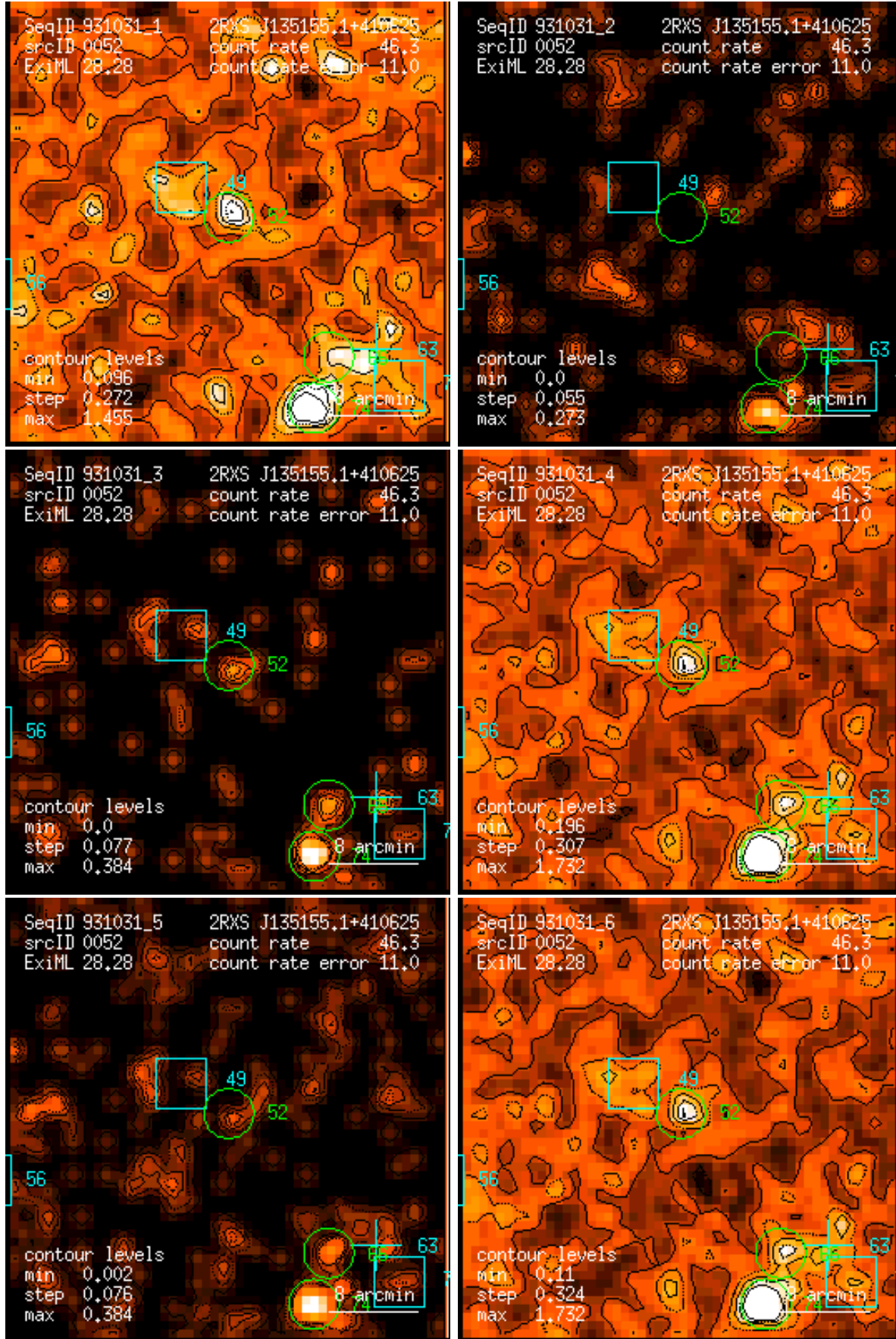
Figure 52: RASS 931031: detection 0052: band rate images, Gaussian filter: (1) PSPC channels 11 – 41, (2) 52 – 90, (3) 91 – 201, (4) 11 – 235, (5) 52 – 201, (6) 11 – 201. Broad band rates in counts/ks. Band rate contour levels in counts/ks/arcmin 2 .
