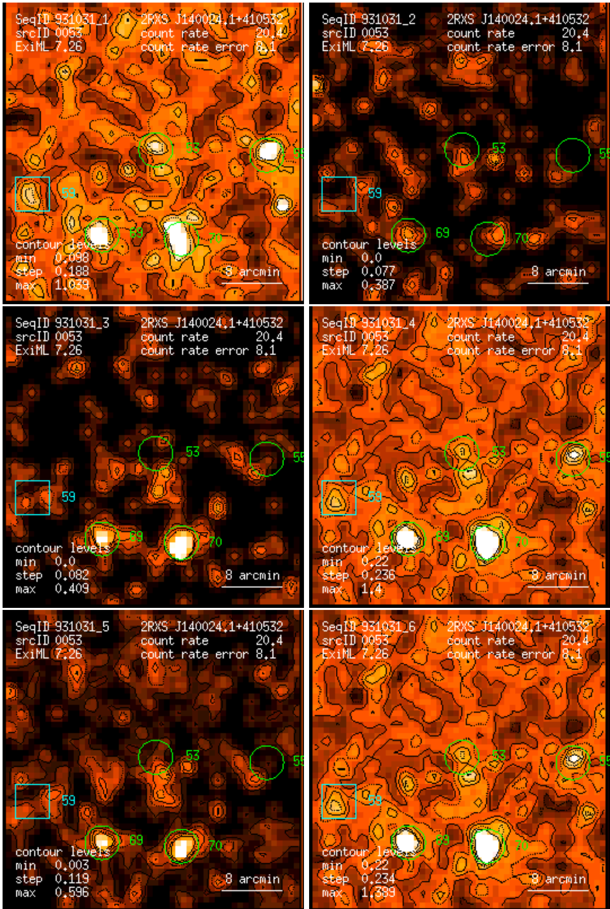
Figure 53: RASS 931031: detection 0053: band rate images, Gaussian filter: (1) PSPC channels 11 – 41, (2) 52 – 90, (3) 91 – 201, (4) 11 – 235, (5) 52 – 201, (6) 11 – 201. Broad band rates in counts/ks. Band rate contour levels in counts/ks/arcmin 2 .
