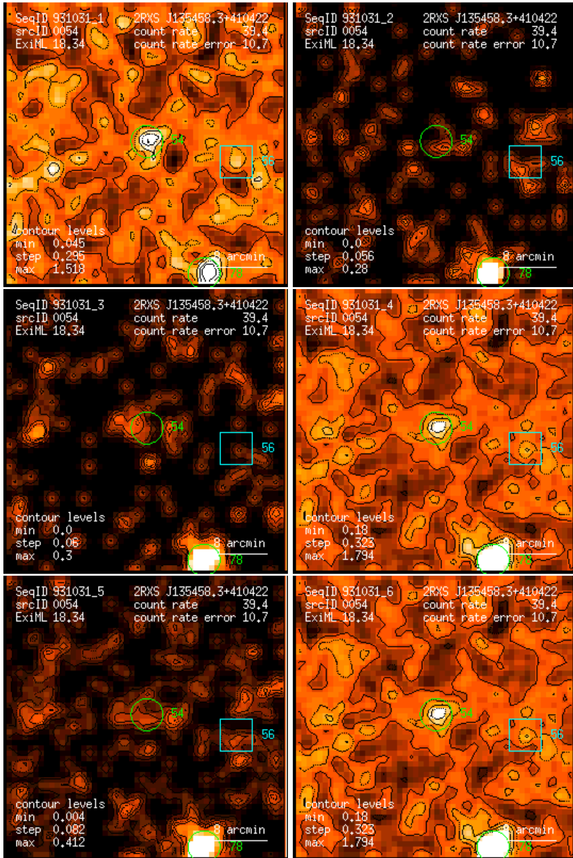
Figure 54: RASS 931031: detection 0054: band rate images, Gaussian filter: (1) PSPC channels 11 – 41, (2) 52 – 90, (3) 91 – 201, (4) 11 – 235, (5) 52 – 201, (6) 11 – 201. Broad band rates in counts/ks. Band rate contour levels in counts/ks/arcmin 2 .
