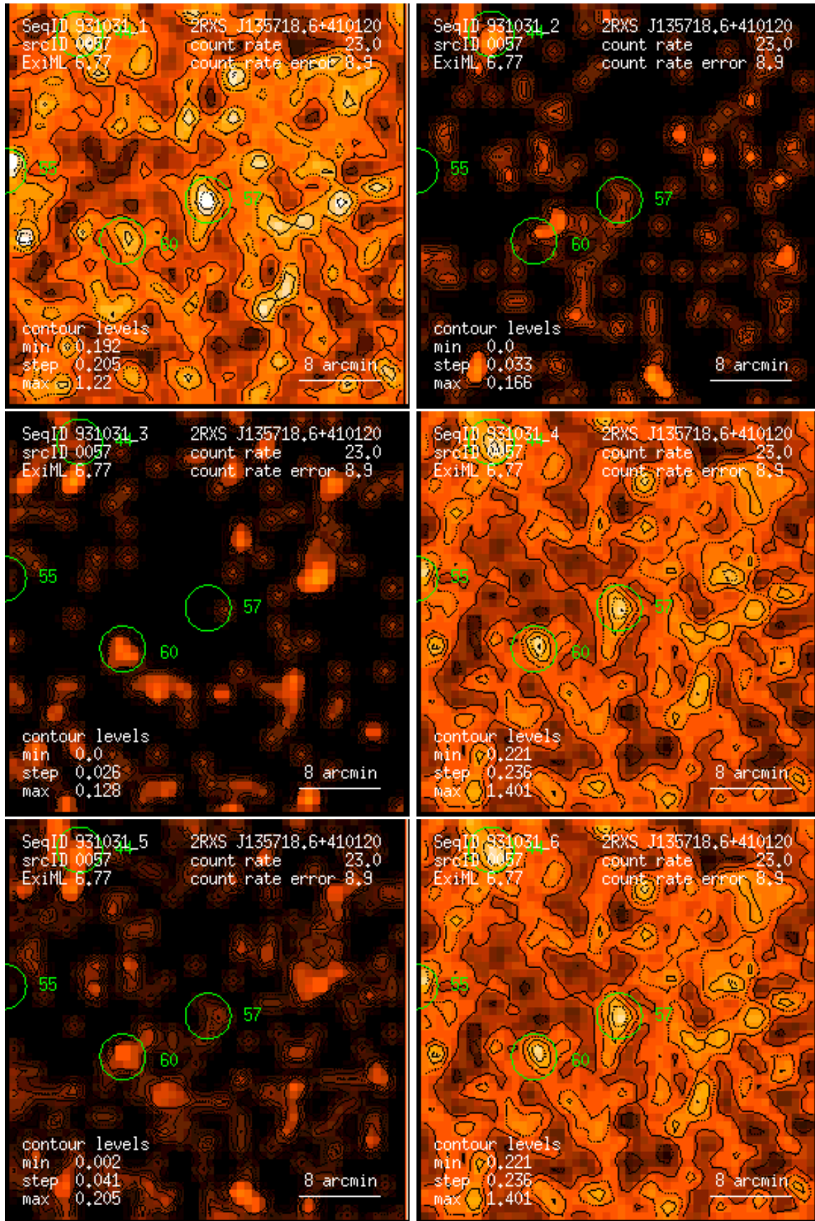
Figure 57: RASS 931031: detection 0057: band rate images, Gaussian filter: (1) PSPC channels 11 – 41, (2) 52 – 90, (3) 91 – 201, (4) 11 – 235, (5) 52 – 201, (6) 11 – 201. Broad band rates in counts/ks. Band rate contour levels in counts/ks/arcmin 2 .
