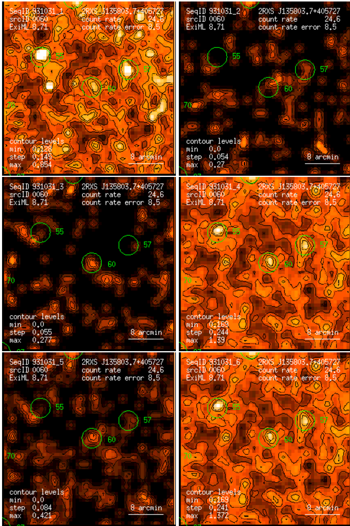
Figure 60: RASS 931031: detection 0060: band rate images, Gaussian filter: (1) PSPC channels 11 – 41, (2) 52 – 90, (3) 91 – 201, (4) 11 – 235, (5) 52 – 201, (6) 11 – 201. Broad band rates in counts/ks. Band rate contour levels in counts/ks/arcmin 2 .
