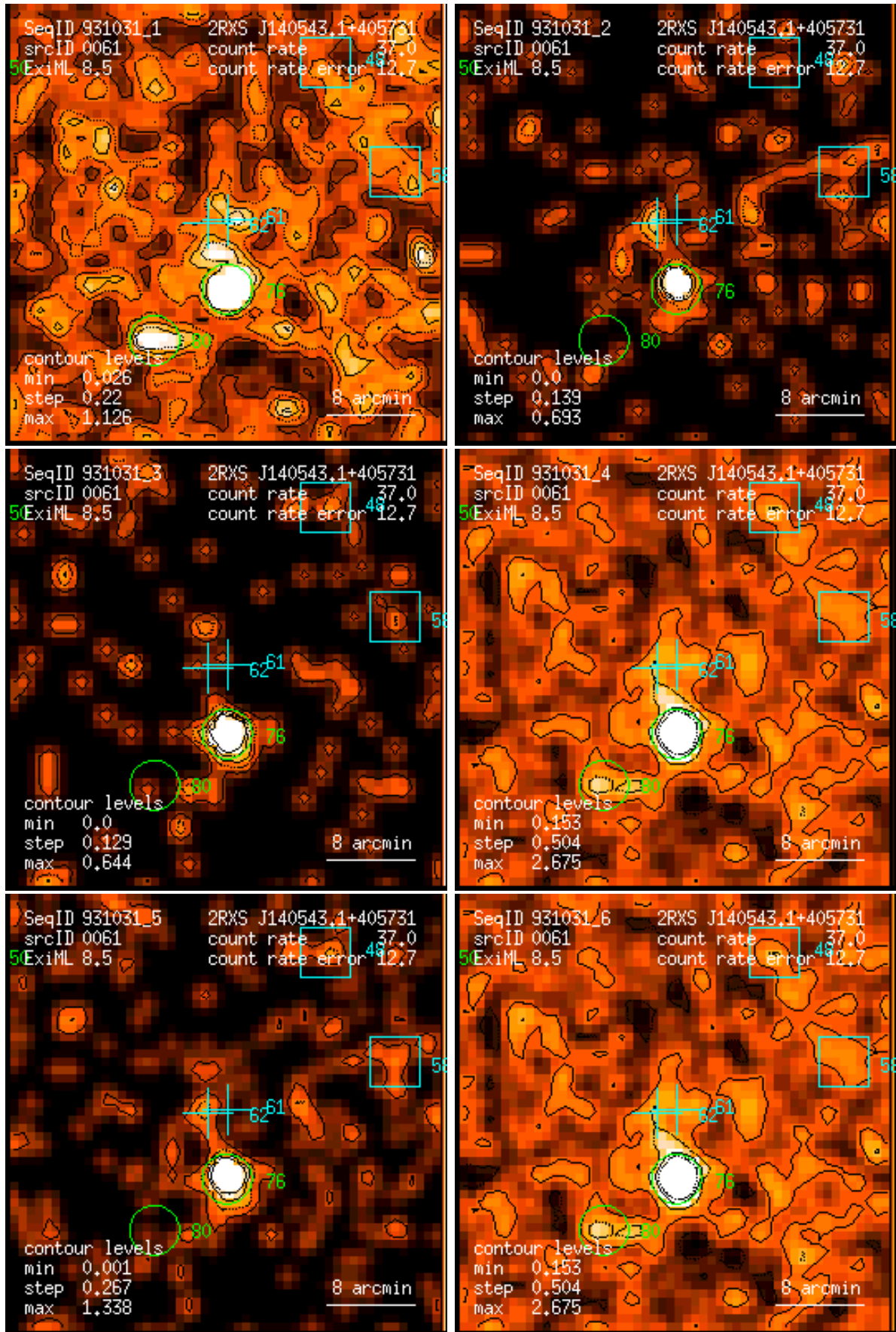
Figure 61: RASS 931031: detection 0061: band rate images, Gaussian filter: (1) PSPC channels 11 – 41, (2) 52 – 90, (3) 91 – 201, (4) 11 – 235, (5) 52 – 201, (6) 11 – 201. Broad band rates in counts/ks. Band rate contour levels in counts/ks/arcmin 2 .
