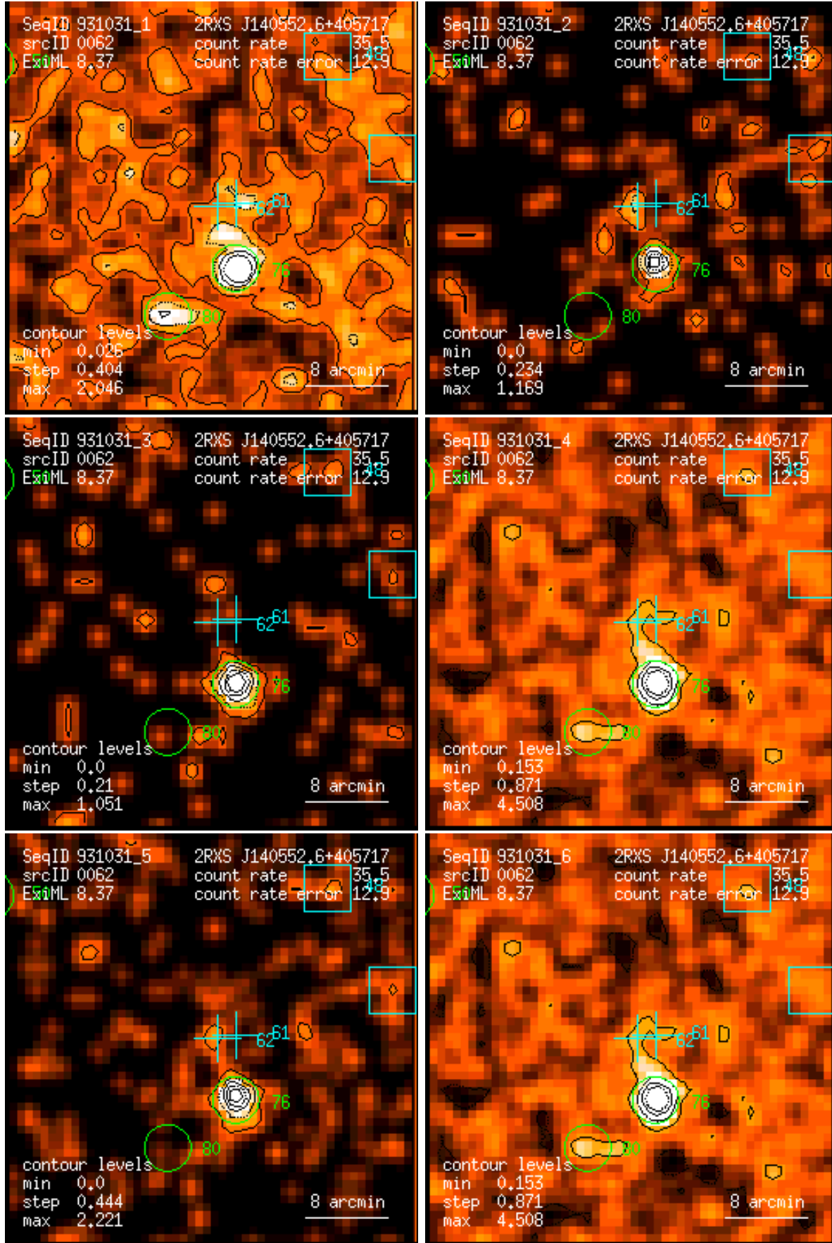
Figure 62: RASS 931031: detection 0062: band rate images, Gaussian filter: (1) PSPC channels 11 – 41, (2) 52 – 90, (3) 91 – 201, (4) 11 – 235, (5) 52 – 201, (6) 11 – 201. Broad band rates in counts/ks. Band rate contour levels in counts/ks/arcmin 2 .
