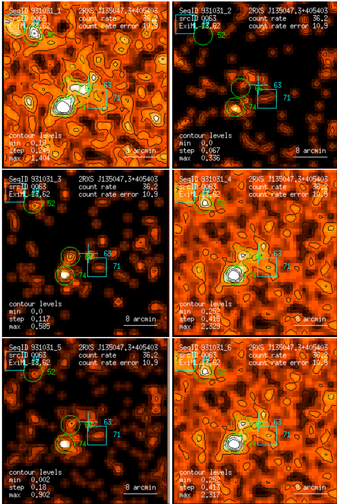
Figure 63: RASS 931031: detection 0063: band rate images, Gaussian filter: (1) PSPC channels 11 – 41, (2) 52 – 90, (3) 91 – 201, (4) 11 – 235, (5) 52 – 201, (6) 11 – 201. Broad band rates in counts/ks. Band rate contour levels in counts/ks/arcmin 2 .
