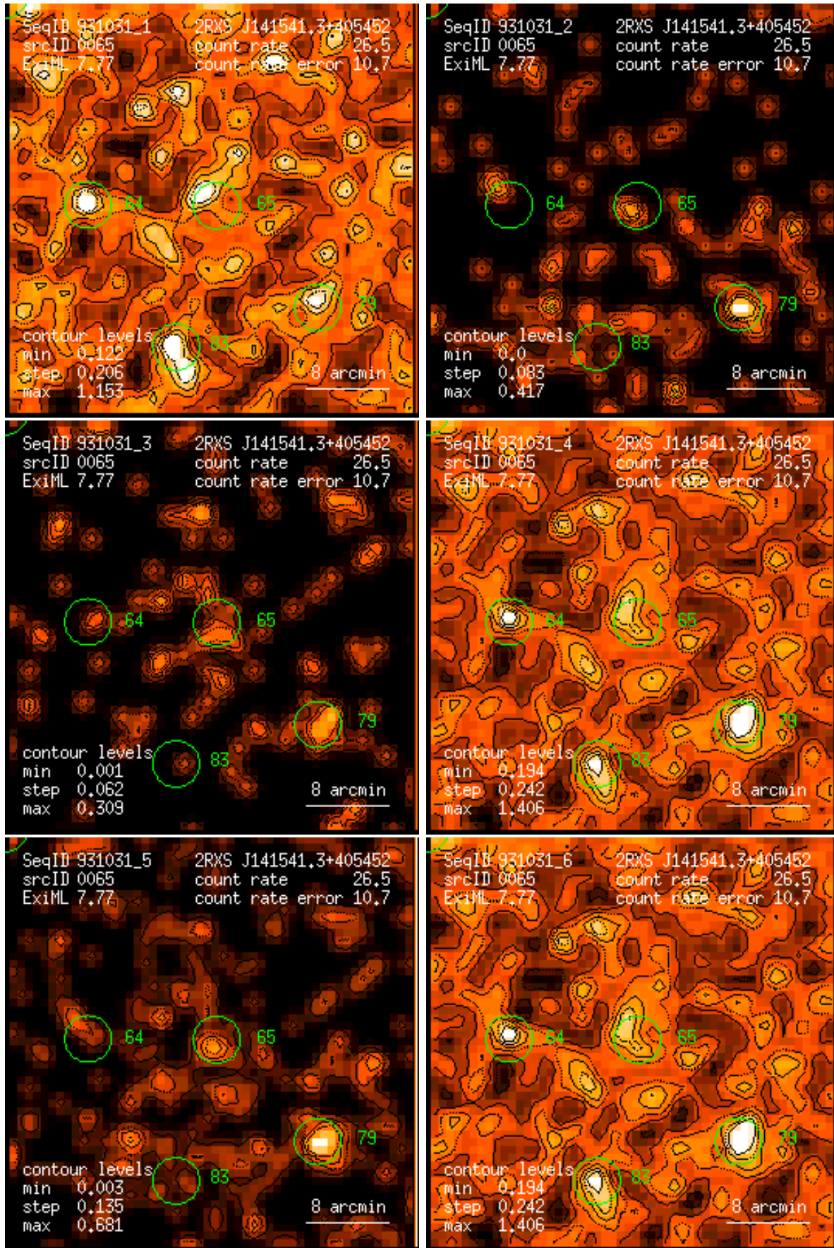
Figure 65: RASS 931031: detection 0065: band rate images, Gaussian filter: (1) PSPC channels 11 – 41, (2) 52 – 90, (3) 91 – 201, (4) 11 – 235, (5) 52 – 201, (6) 11 – 201. Broad band rates in counts/ks. Band rate contour levels in counts/ks/arcmin 2 .
