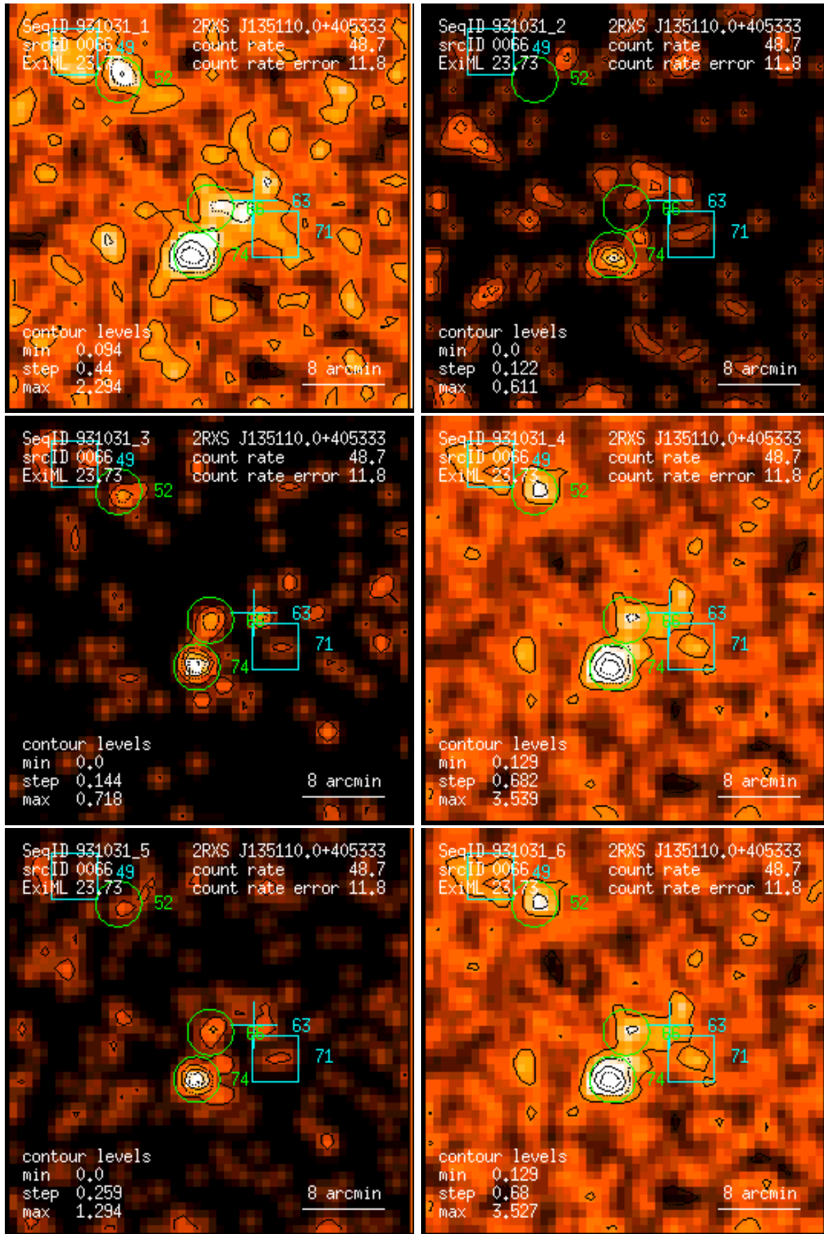
Figure 66: RASS 931031: detection 0066: band rate images, Gaussian filter: (1) PSPC channels 11 – 41, (2) 52 – 90, (3) 91 – 201, (4) 11 – 235, (5) 52 – 201, (6) 11 – 201. Broad band rates in counts/ks. Band rate contour levels in counts/ks/arcmin 2 .
