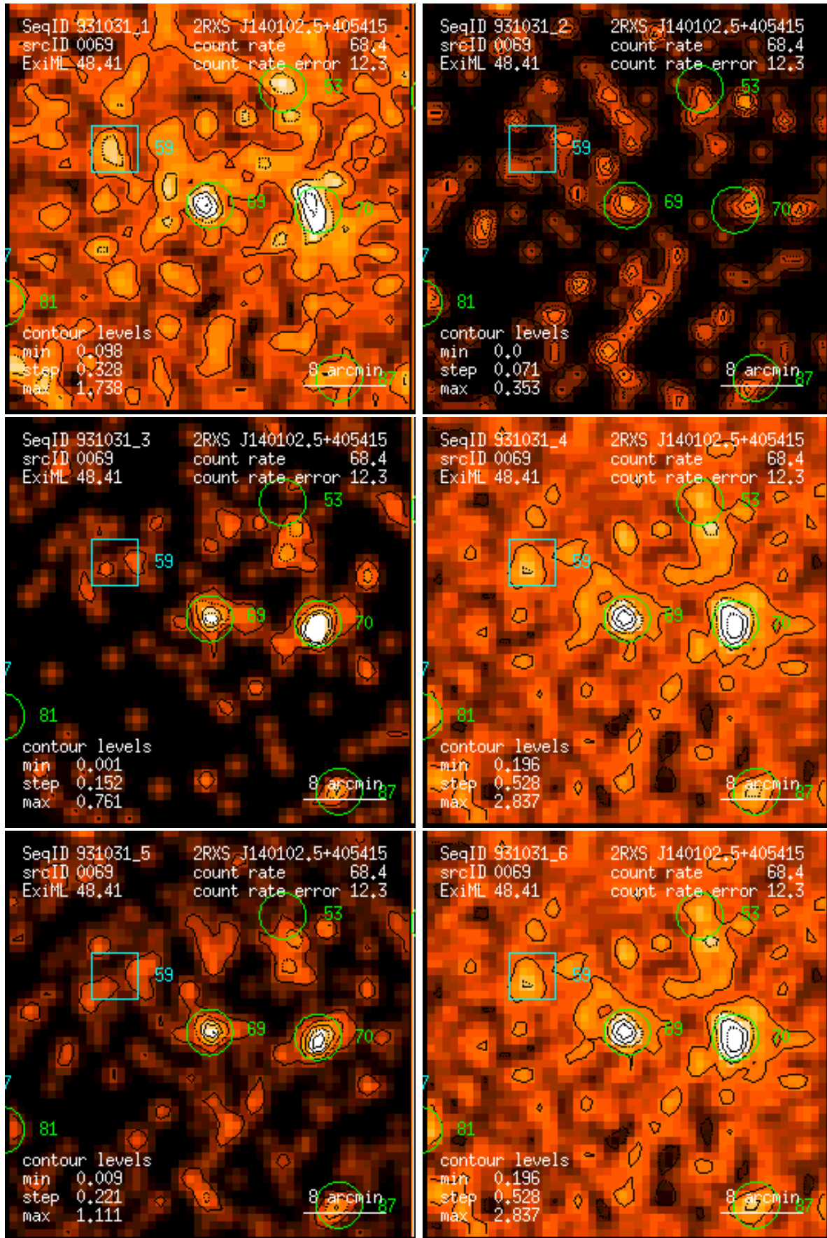
Figure 69: RASS 931031: detection 0069: band rate images, Gaussian filter: (1) PSPC channels 11 – 41, (2) 52 – 90, (3) 91 – 201, (4) 11 – 235, (5) 52 – 201, (6) 11 – 201. Broad band rates in counts/ks. Band rate contour levels in counts/ks/arcmin 2 .
