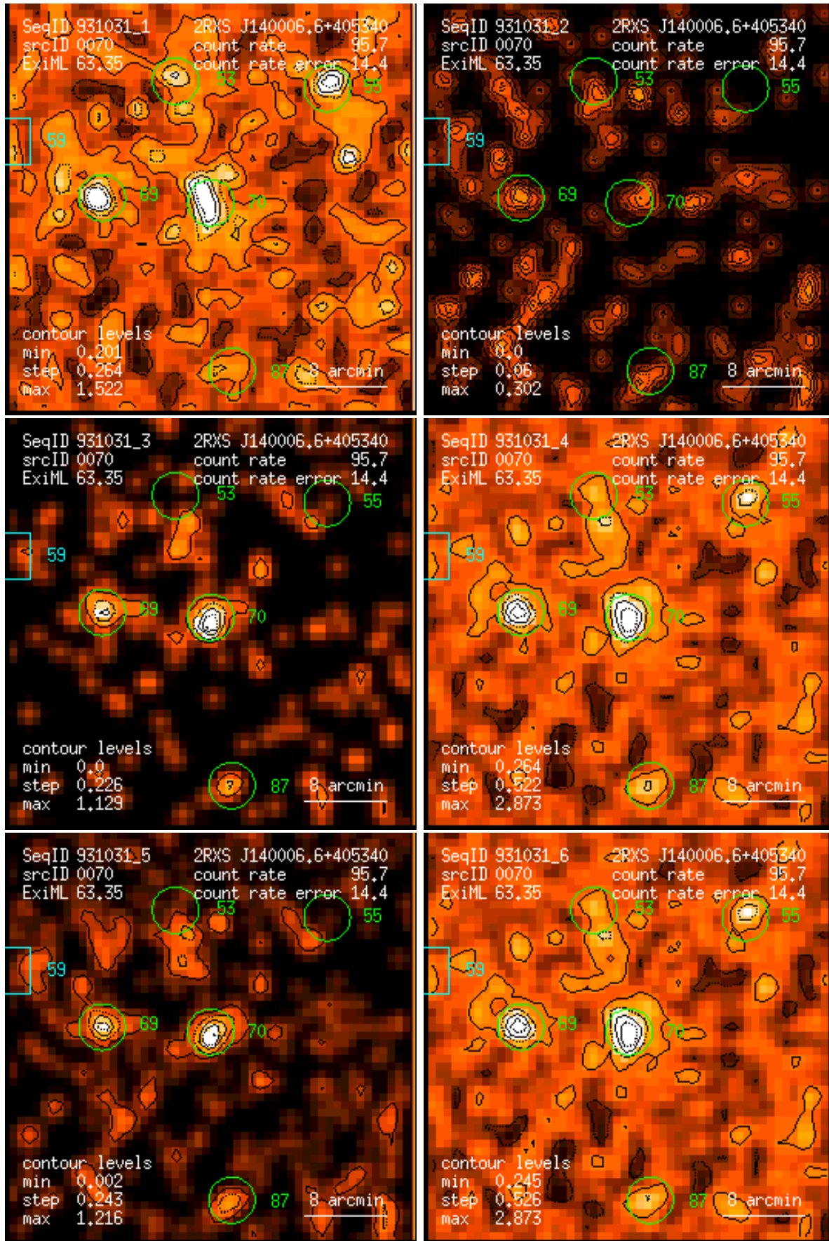
Figure 70: RASS 931031: detection 0070: band rate images, Gaussian filter: (1) PSPC channels 11 – 41, (2) 52 – 90, (3) 91 – 201, (4) 11 – 235, (5) 52 – 201, (6) 11 – 201. Broad band rates in counts/ks. Band rate contour levels in counts/ks/arcmin 2 .
