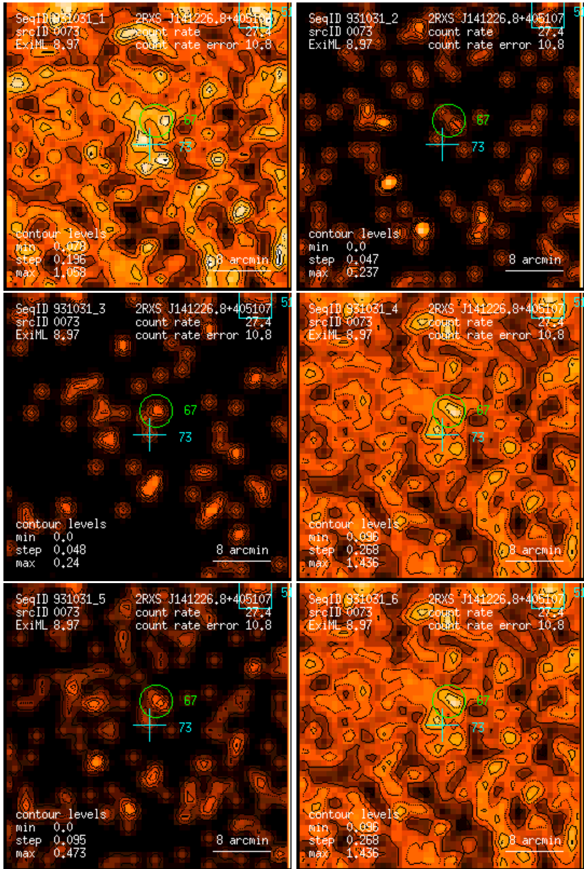
Figure 73: RASS 931031: detection 0073: band rate images, Gaussian filter: (1) PSPC channels 11 – 41, (2) 52 – 90, (3) 91 – 201, (4) 11 – 235, (5) 52 – 201, (6) 11 – 201. Broad band rates in counts/ks. Band rate contour levels in counts/ks/arcmin 2 .
