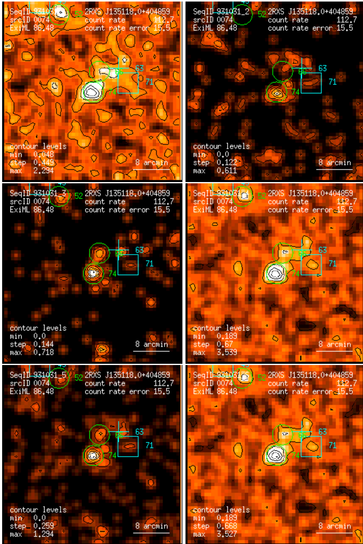
Figure 74: RASS 931031: detection 0074: band rate images, Gaussian filter: (1) PSPC channels 11 – 41, (2) 52 – 90, (3) 91 – 201, (4) 11 – 235, (5) 52 – 201, (6) 11 – 201. Broad band rates in counts/ks. Band rate contour levels in counts/ks/arcmin 2 .
