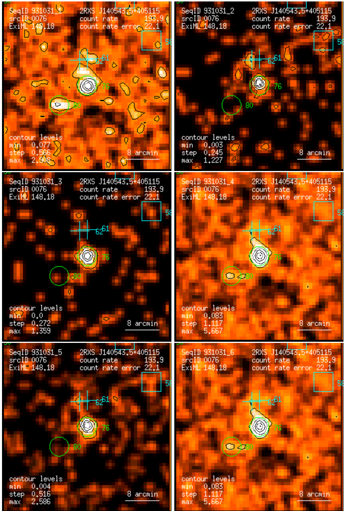
Figure 76: RASS 931031: detection 0076: band rate images, Gaussian filter: (1) PSPC channels 11 – 41, (2) 52 – 90, (3) 91 – 201, (4) 11 – 235, (5) 52 – 201, (6) 11 – 201. Broad band rates in counts/ks. Band rate contour levels in counts/ks/arcmin 2 .
