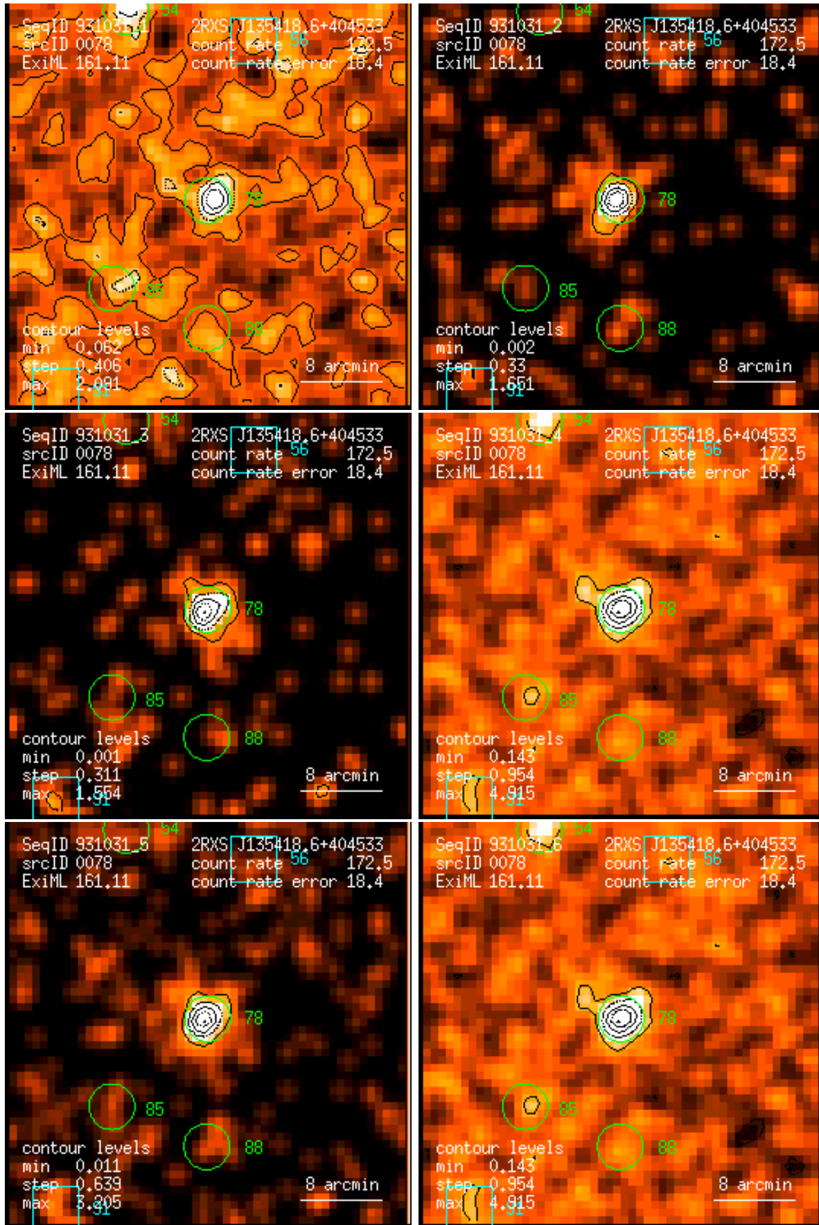
Figure 78: RASS 931031: detection 0078: band rate images, Gaussian filter: (1) PSPC channels 11 – 41, (2) 52 – 90, (3) 91 – 201, (4) 11 – 235, (5) 52 – 201, (6) 11 – 201. Broad band rates in counts/ks. Band rate contour levels in counts/ks/arcmin 2 .
