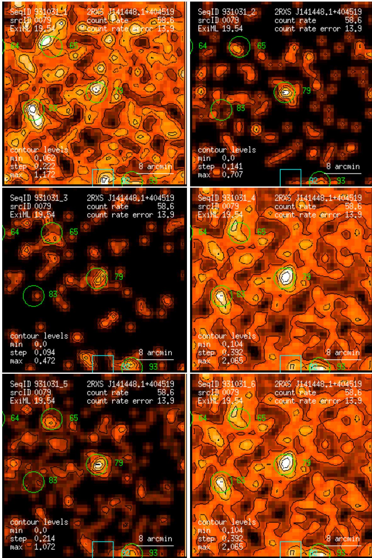
Figure 79: RASS 931031: detection 0079: band rate images, Gaussian filter: (1) PSPC channels 11 – 41, (2) 52 – 90, (3) 91 – 201, (4) 11 – 235, (5) 52 – 201, (6) 11 – 201. Broad band rates in counts/ks. Band rate contour levels in counts/ks/arcmin 2 .
