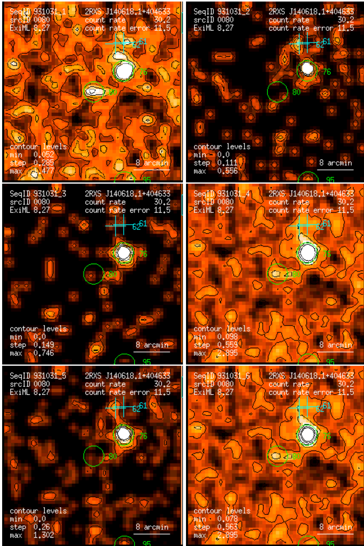
Figure 80: RASS 931031: detection 0080: band rate images, Gaussian filter: (1) PSPC channels 11 – 41, (2) 52 – 90, (3) 91 – 201, (4) 11 – 235, (5) 52 – 201, (6) 11 – 201. Broad band rates in counts/ks. Band rate contour levels in counts/ks/arcmin 2 .
